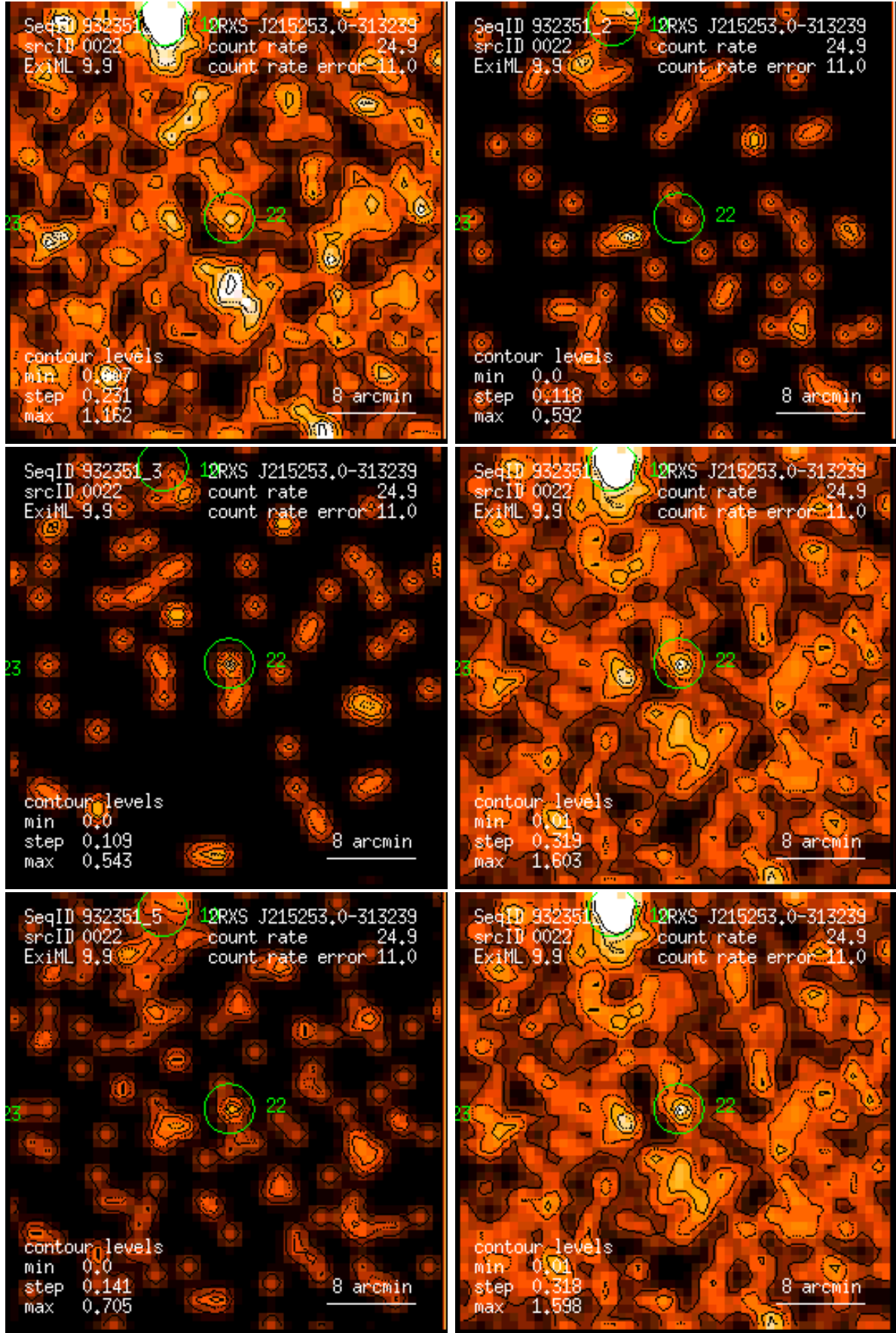
Figure 22: RASS 932351: detection 0022: band rate images, Gaussian filter: (1) PSPC channels 11 – 41, (2) 52 – 90, (3) 91 – 201, (4) 11 – 235, (5) 52 – 201, (6) 11 – 201. Broad band rates in counts/ks. Band rate contour levels in counts/ks/arcmin 2 .
