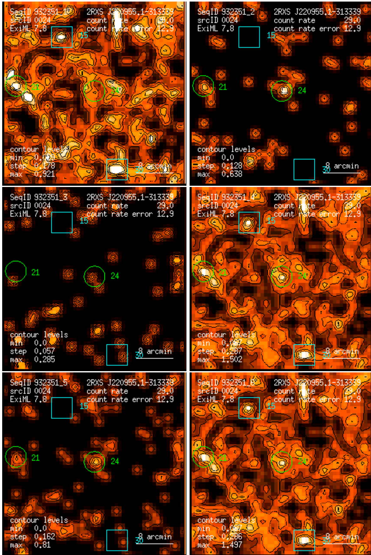
Figure 24: RASS 932351: detection 0024: band rate images, Gaussian filter: (1) PSPC channels 11 – 41, (2) 52 – 90, (3) 91 – 201, (4) 11 – 235, (5) 52 – 201, (6) 11 – 201. Broad band rates in counts/ks. Band rate contour levels in counts/ks/arcmin 2 .
