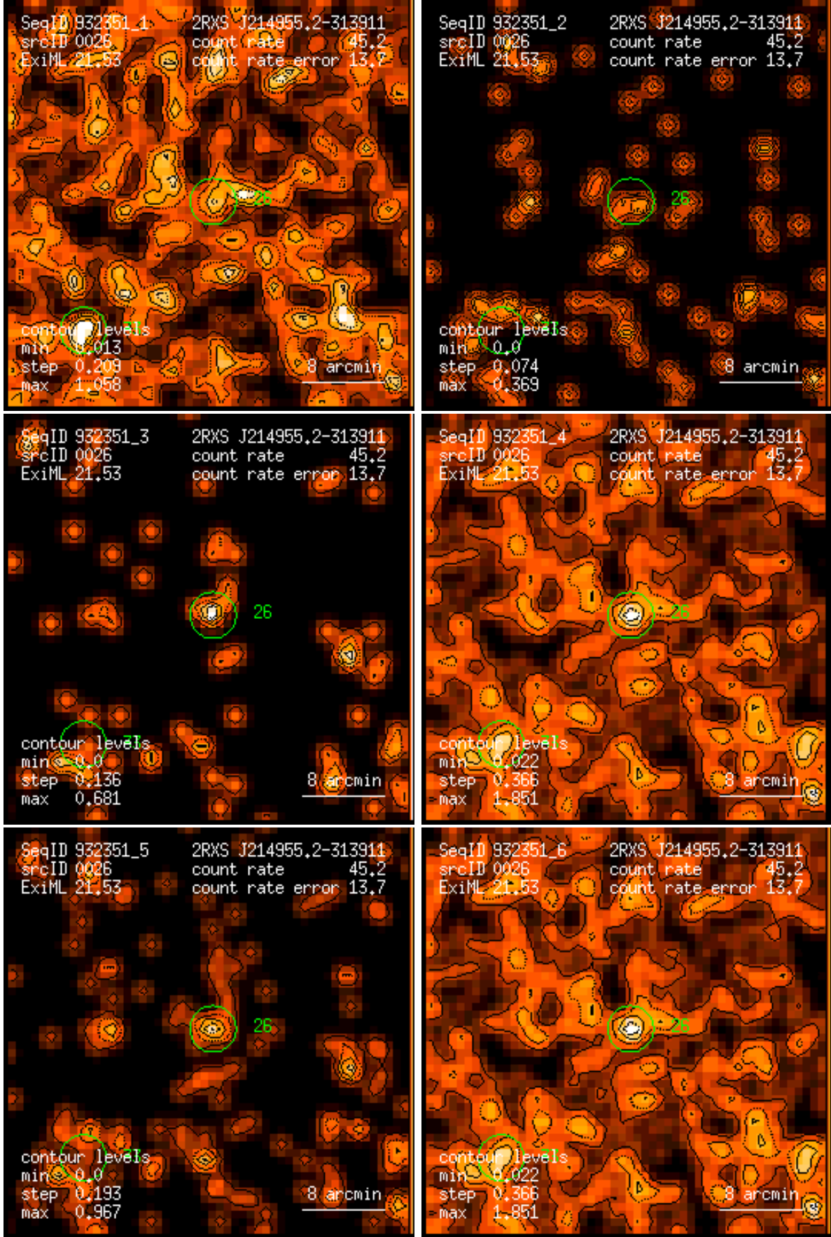
Figure 26: RASS 932351: detection 0026: band rate images, Gaussian filter: (1) PSPC channels 11 – 41, (2) 52 – 90, (3) 91 – 201, (4) 11 – 235, (5) 52 – 201, (6) 11 – 201. Broad band rates in counts/ks. Band rate contour levels in counts/ks/arcmin 2 .
