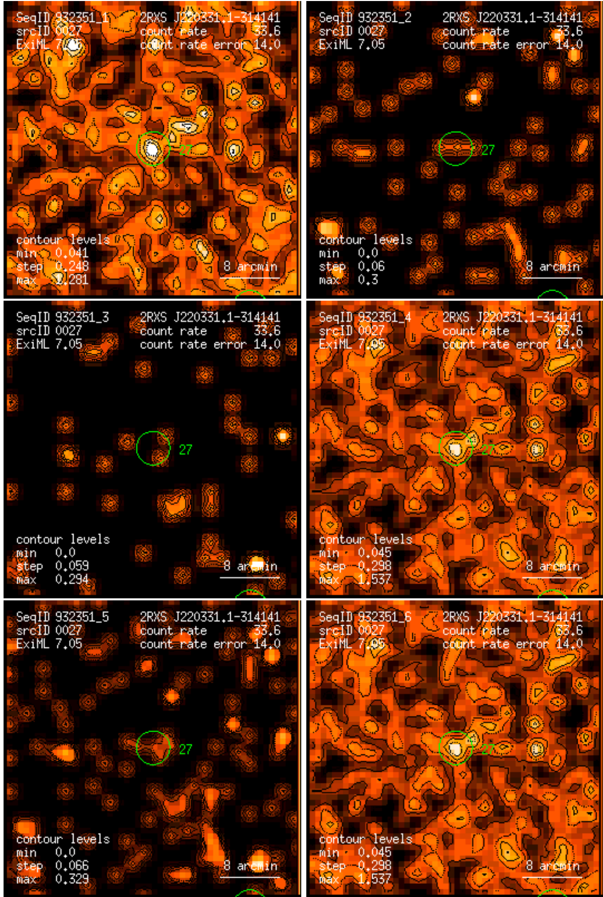
Figure 27: RASS 932351: detection 0027: band rate images, Gaussian filter: (1) PSPC channels 11 – 41, (2) 52 – 90, (3) 91 – 201, (4) 11 – 235, (5) 52 – 201, (6) 11 – 201. Broad band rates in counts/ks. Band rate contour levels in counts/ks/arcmin 2 .
