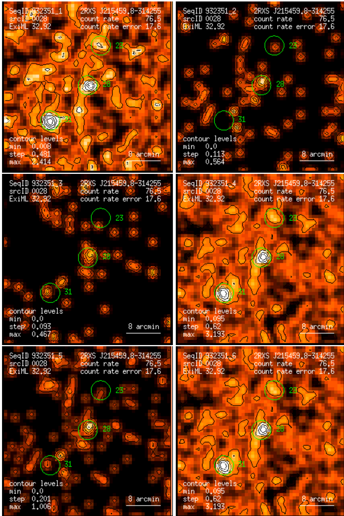
Figure 28: RASS 932351: detection 0028: band rate images, Gaussian filter: (1) PSPC channels 11 – 41, (2) 52 – 90, (3) 91 – 201, (4) 11 – 235, (5) 52 – 201, (6) 11 – 201. Broad band rates in counts/ks. Band rate contour levels in counts/ks/arcmin 2 .
