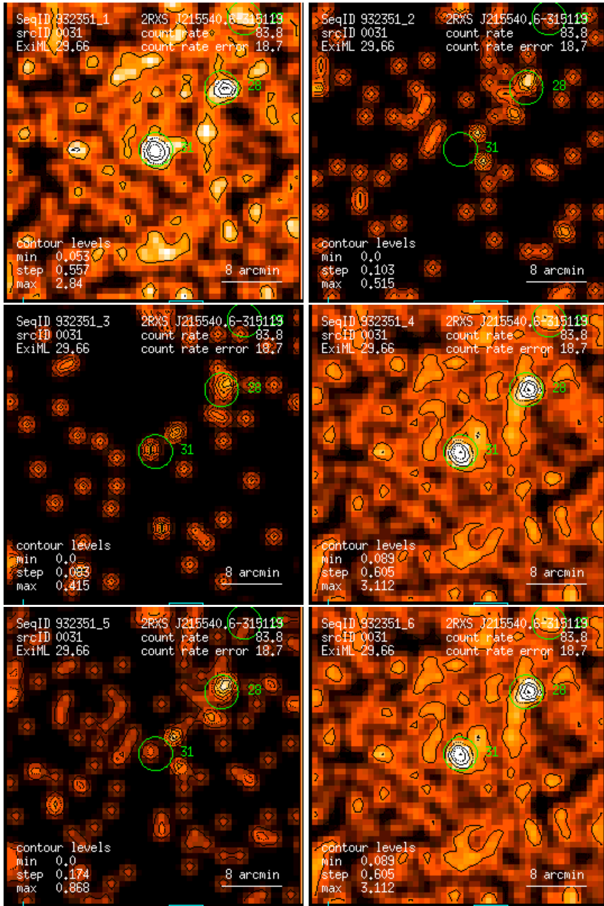
Figure 31: RASS 932351: detection 0031: band rate images, Gaussian filter: (1) PSPC channels 11 – 41, (2) 52 – 90, (3) 91 – 201, (4) 11 – 235, (5) 52 – 201, (6) 11 – 201. Broad band rates in counts/ks. Band rate contour levels in counts/ks/arcmin 2 .
