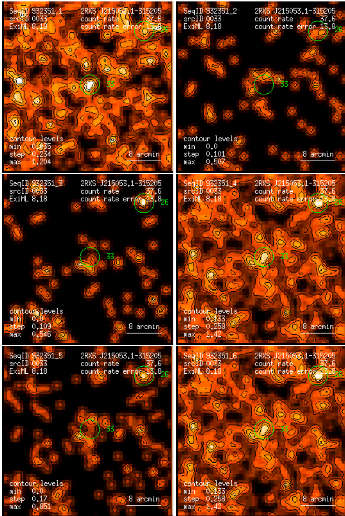
Figure 33: RASS 932351: detection 0033: band rate images, Gaussian filter: (1) PSPC channels 11 – 41, (2) 52 – 90, (3) 91 – 201, (4) 11 – 235, (5) 52 – 201, (6) 11 – 201. Broad band rates in counts/ks. Band rate contour levels in counts/ks/arcmin 2 .
