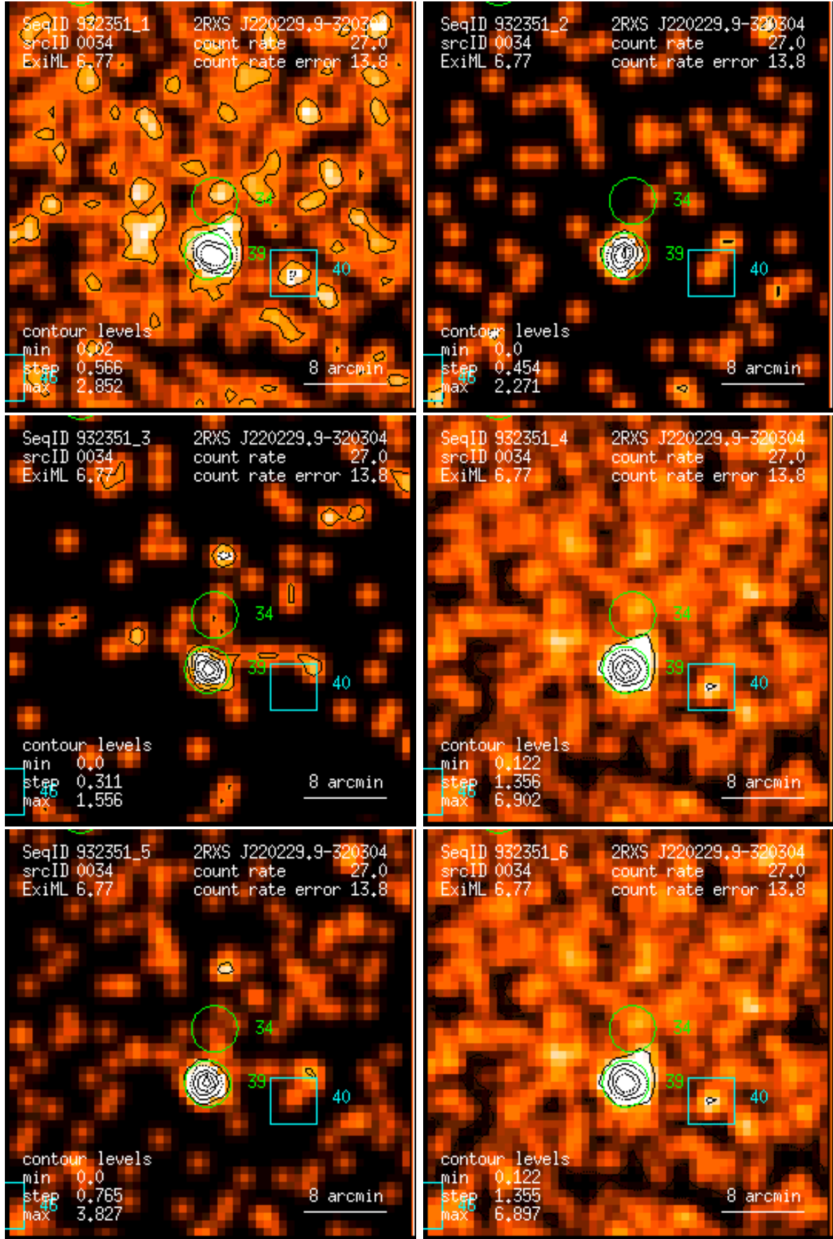
Figure 34: RASS 932351: detection 0034: band rate images, Gaussian filter: (1) PSPC channels 11 – 41, (2) 52 – 90, (3) 91 – 201, (4) 11 – 235, (5) 52 – 201, (6) 11 – 201. Broad band rates in counts/ks. Band rate contour levels in counts/ks/arcmin 2 .
