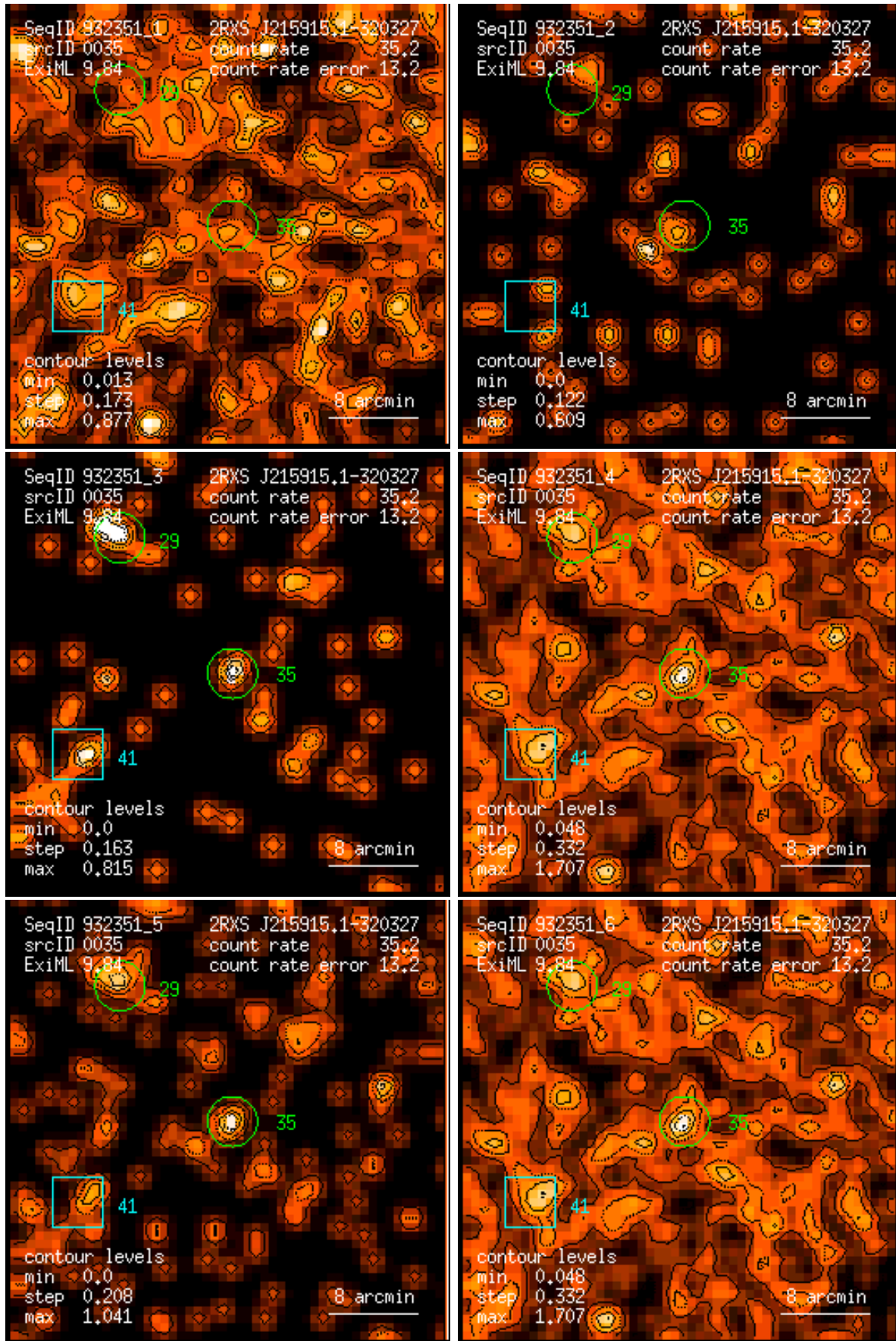
Figure 35: RASS 932351: detection 0035: band rate images, Gaussian filter: (1) PSPC channels 11 – 41, (2) 52 – 90, (3) 91 – 201, (4) 11 – 235, (5) 52 – 201, (6) 11 – 201. Broad band rates in counts/ks. Band rate contour levels in counts/ks/arcmin 2 .
