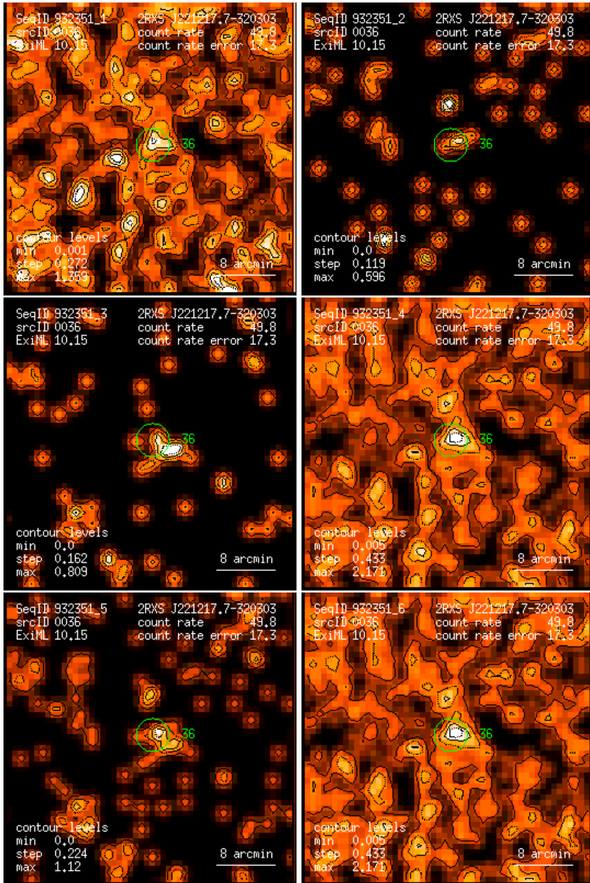
Figure 36: RASS 932351: detection 0036: band rate images, Gaussian filter: (1) PSPC channels 11 – 41, (2) 52 – 90, (3) 91 – 201, (4) 11 – 235, (5) 52 – 201, (6) 11 – 201. Broad band rates in counts/ks. Band rate contour levels in counts/ks/arcmin 2 .
