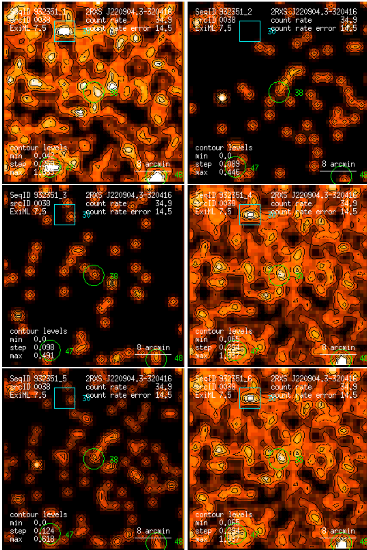
Figure 38: RASS 932351: detection 0038: band rate images, Gaussian filter: (1) PSPC channels 11 – 41, (2) 52 – 90, (3) 91 – 201, (4) 11 – 235, (5) 52 – 201, (6) 11 – 201. Broad band rates in counts/ks. Band rate contour levels in counts/ks/arcmin 2 .
