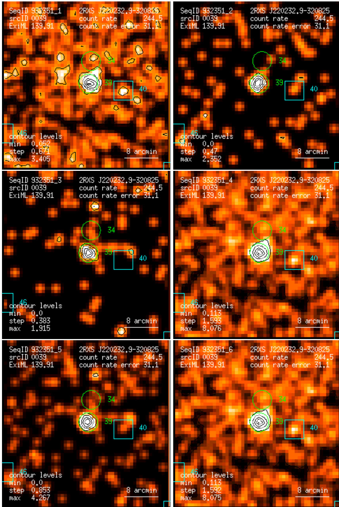
Figure 39: RASS 932351: detection 0039: band rate images, Gaussian filter: (1) PSPC channels 11 – 41, (2) 52 – 90, (3) 91 – 201, (4) 11 – 235, (5) 52 – 201, (6) 11 – 201. Broad band rates in counts/ks. Band rate contour levels in counts/ks/arcmin 2 .
