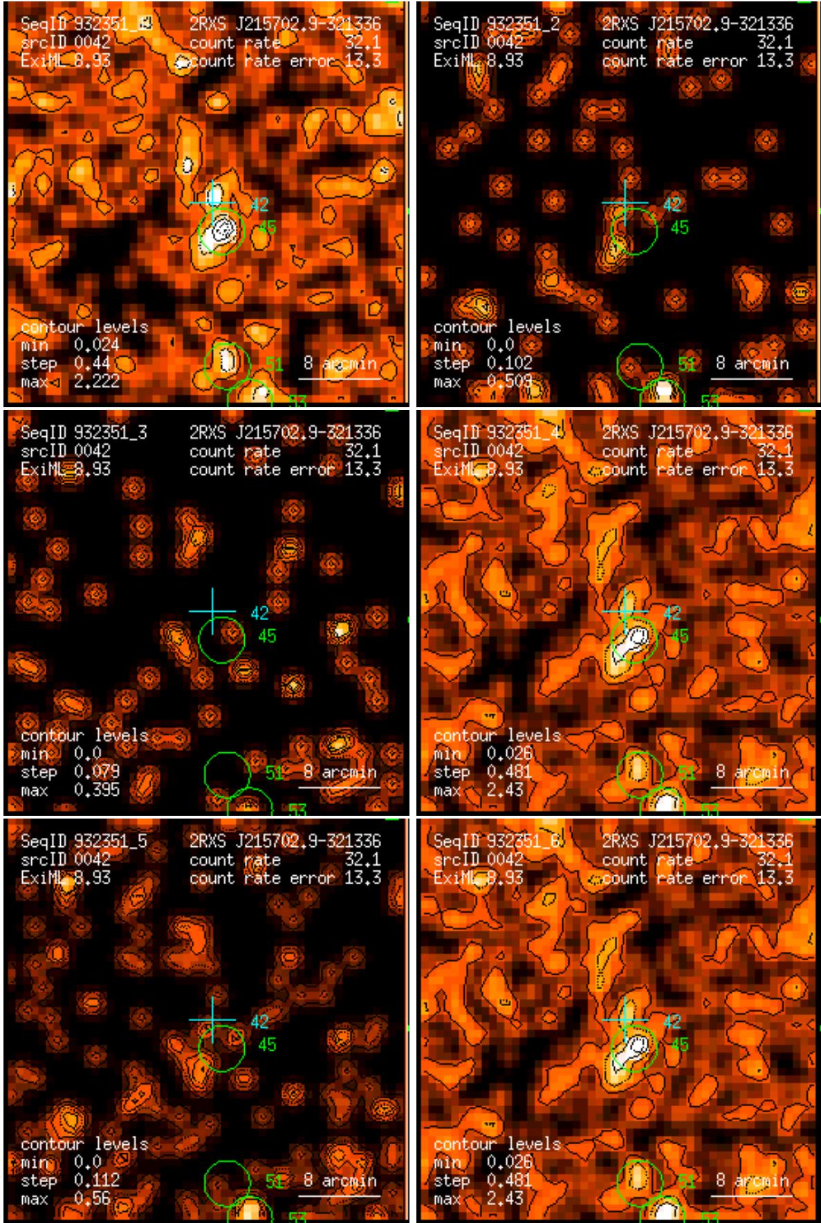
Figure 42: RASS 932351: detection 0042: band rate images, Gaussian filter: (1) PSPPC channels 11 – 41, (2) 52 – 90, (3) 91 – 201, (4) 11 – 235, (5) 52 – 201, (6) 11 – 201. Broad band rates in counts/ks. Band rate contour levels in counts/ks/arcmin 2 .
