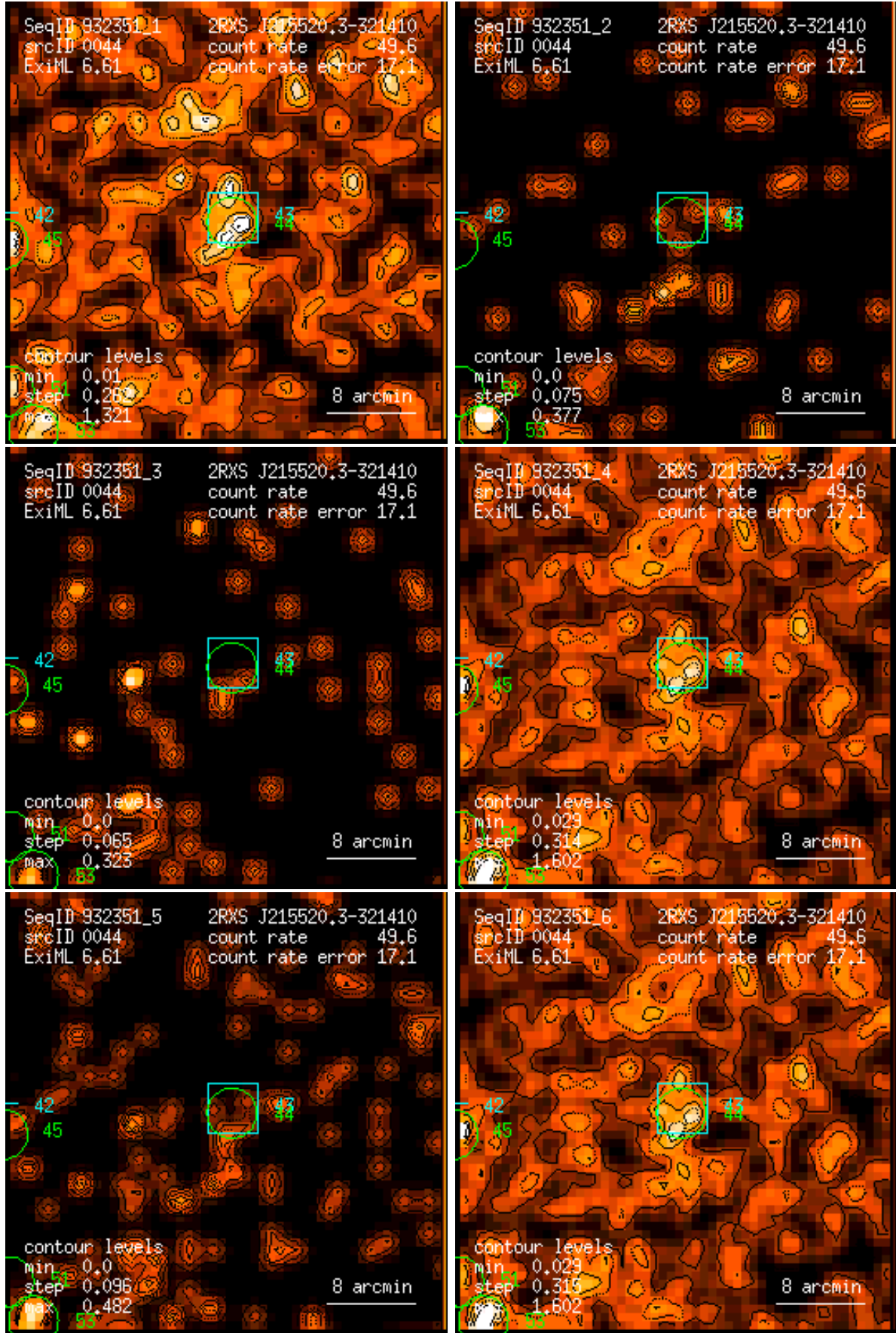
Figure 44: RASS 932351: detection 0044: band rate images, Gaussian filter: (1) PSPC channels 11 – 41, (2) 52 – 90, (3) 91 – 201, (4) 11 – 235, (5) 52 – 201, (6) 11 – 201. Broad band rates in counts/ks. Band rate contour levels in counts/ks/arcmin 2 .
