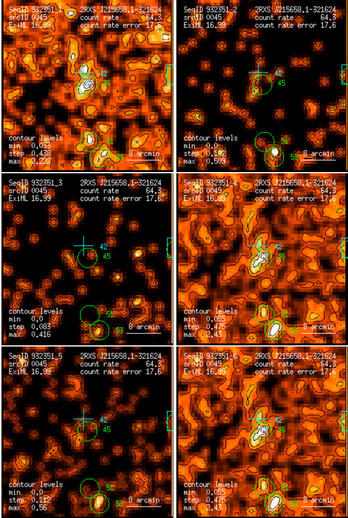
Figure 45: RASS 932351: detection 0045: band rate images, Gaussian filter: (1) PSPC channels 11 – 41, (2) 52 – 90, (3) 91 – 201, (4) 11 – 235, (5) 52 – 201, (6) 11 – 201. Broad band rates in counts/ks. Band rate contour levels in counts/ks/arcmin 2 .
