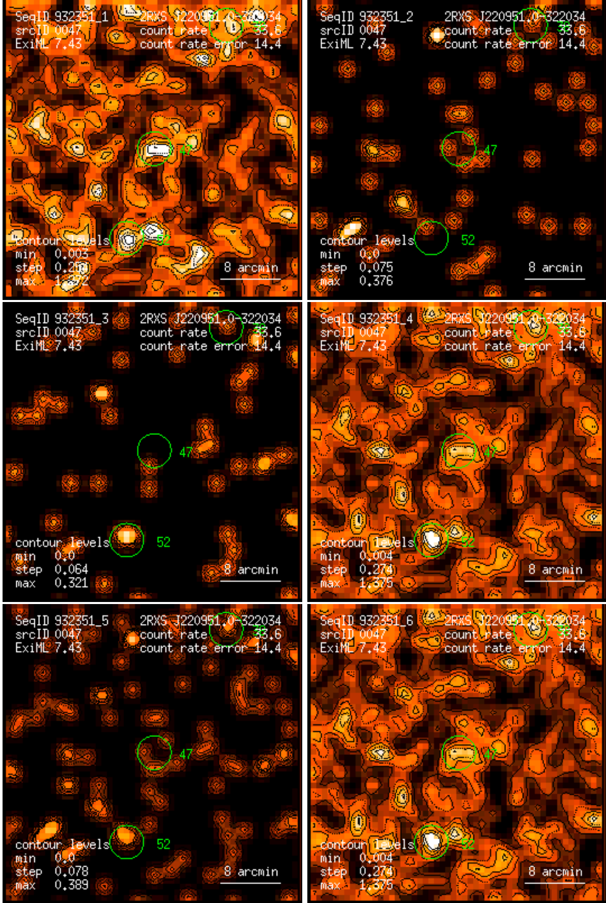
Figure 47: RASS 932351: detection 0047: band rate images, Gaussian filter: (1) PSPC channels 11 – 41, (2) 52 – 90, (3) 91 – 201, (4) 11 – 235, (5) 52 – 201, (6) 11 – 201. Broad band rates in counts/ks. Band rate contour levels in counts/ks/arcmin 2 .
