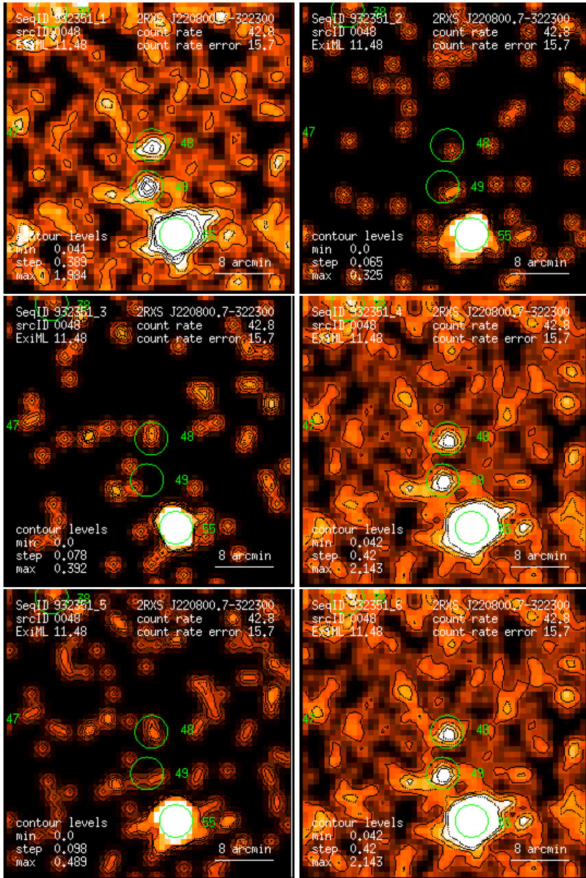
Figure 48: RASS 932351: detection 0048: band rate images, Gaussian filter: (1) PSPC channels 11 – 41, (2) 52 – 90, (3) 91 – 201, (4) 11 – 235, (5) 52 – 201, (6) 11 – 201. Broad band rates in counts/ks. Band rate contour levels in counts/ks/arcmin 2 .
