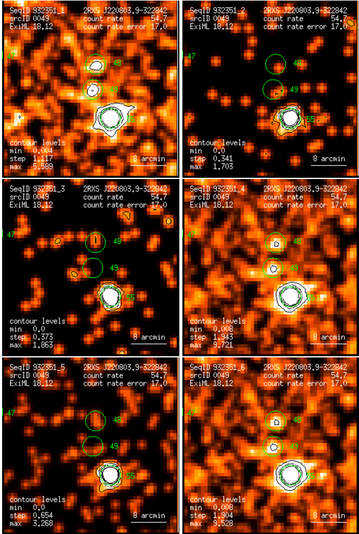
Figure 49: RASS 932351: detection 0049: band rate images, Gaussian filter: (1) PSPC channels 11 – 41, (2) 52 – 90, (3) 91 – 201, (4) 11 – 235, (5) 52 – 201, (6) 11 – 201. Broad band rates in counts/ks. Band rate contour levels in counts/ks/arcmin 2 .
