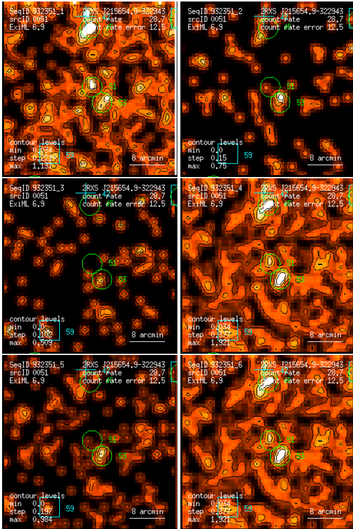
Figure 51: RASS 932351: detection 0051: band rate images, Gaussian filter: (1) PSPC channels 11 – 41, (2) 52 – 90, (3) 91 – 201, (4) 11 – 235, (5) 52 – 201, (6) 11 – 201. Broad band rates in counts/ks. Band rate contour levels in counts/ks/arcmin 2 .
