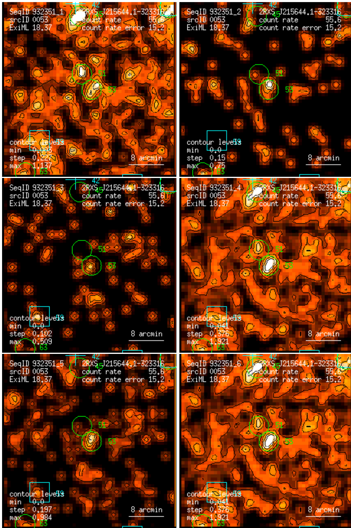
Figure 53: RASS 932351: detection 0053: band rate images, Gaussian filter: (1) PSPC channels 11 – 41, (2) 52 – 90, (3) 91 – 201, (4) 11 – 235, (5) 52 – 201, (6) 11 – 201. Broad band rates in counts/ks. Band rate contour levels in counts/ks/arcmin 2 .
