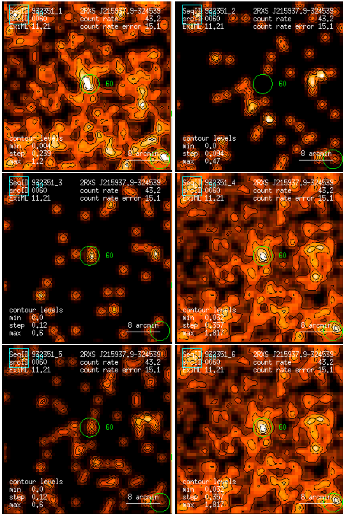
Figure 60: RASS 932351: detection 0060: band rate images, Gaussian filter: (1) PSPC channels 11 – 41, (2) 52 – 90, (3) 91 – 201, (4) 11 – 235, (5) 52 – 201, (6) 11 – 201. Broad band rates in counts/ks. Band rate contour levels in counts/ks/arcmin 2 .
