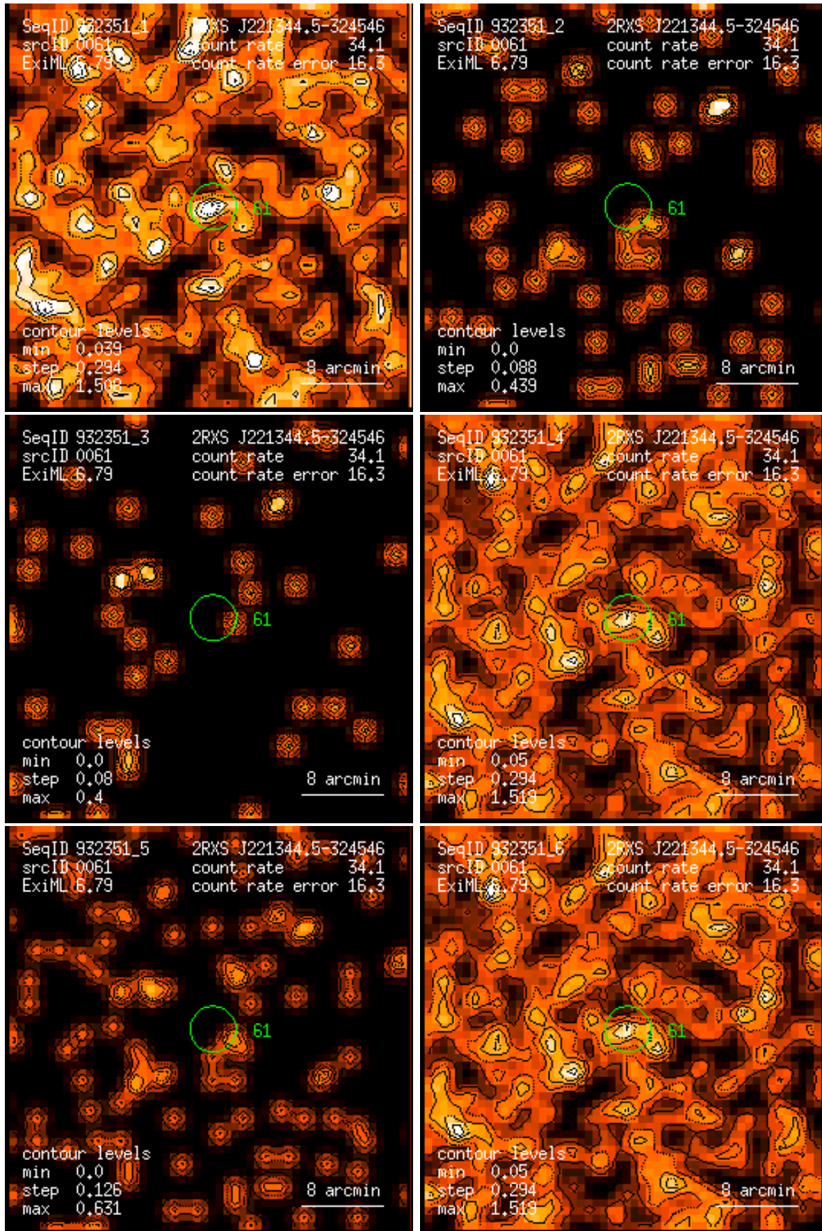
Figure 61: RASS 932351: detection 0061: band rate images, Gaussian filter: (1) PSPC channels 11 – 41, (2) 52 – 90, (3) 91 – 201, (4) 11 – 235, (5) 52 – 201, (6) 11 – 201. Broad band rates in counts/ks. Band rate contour levels in counts/ks/arcmin 2 .
