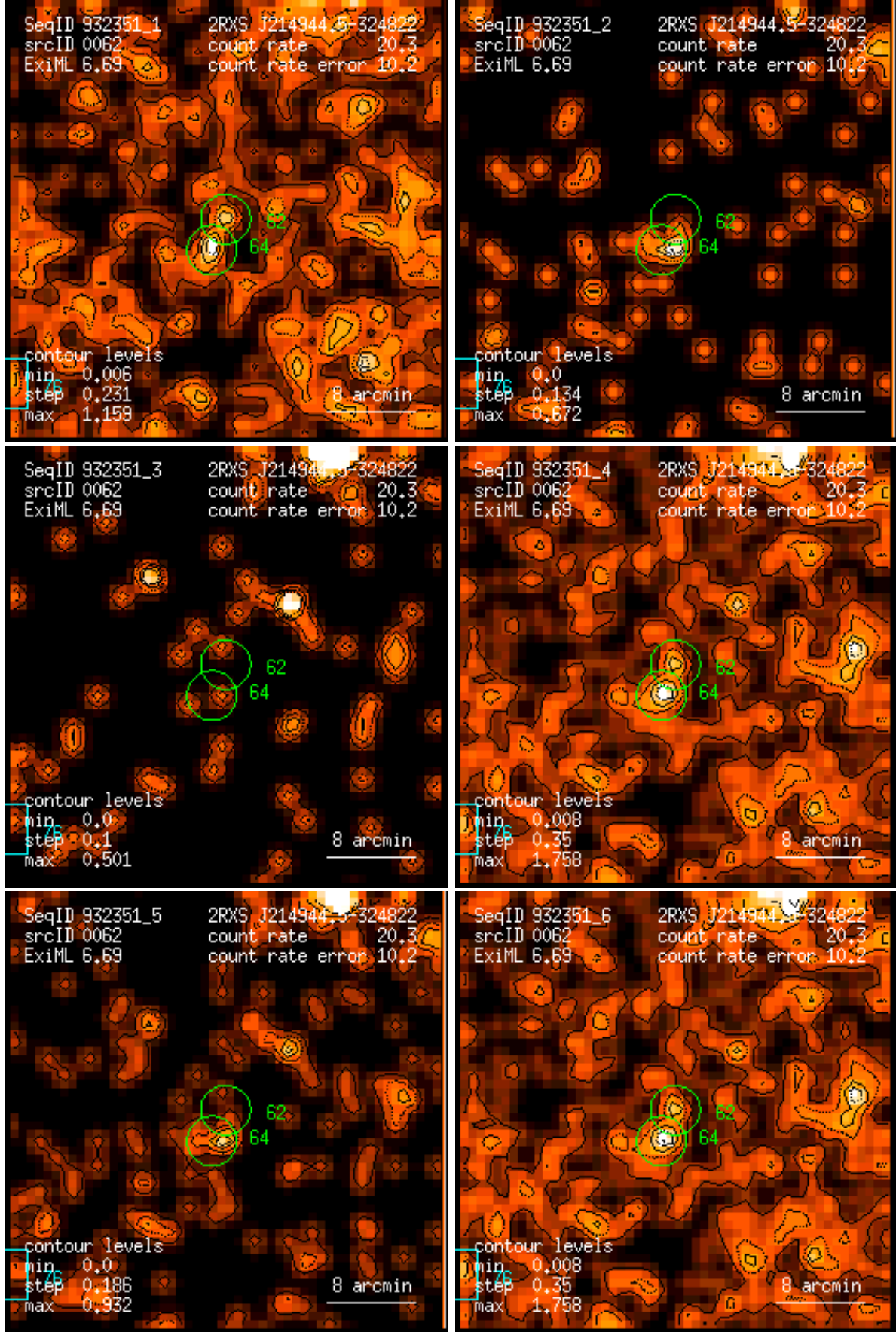
Figure 62: RASS 932351: detection 0062: band rate images, Gaussian filter: (1) PSPC channels 11 – 41, (2) 52 – 90, (3) 91 – 201, (4) 11 – 235, (5) 52 – 201, (6) 11 – 201. Broad band rates in counts/ks. Band rate contour levels in counts/ks/arcmin 2 .
