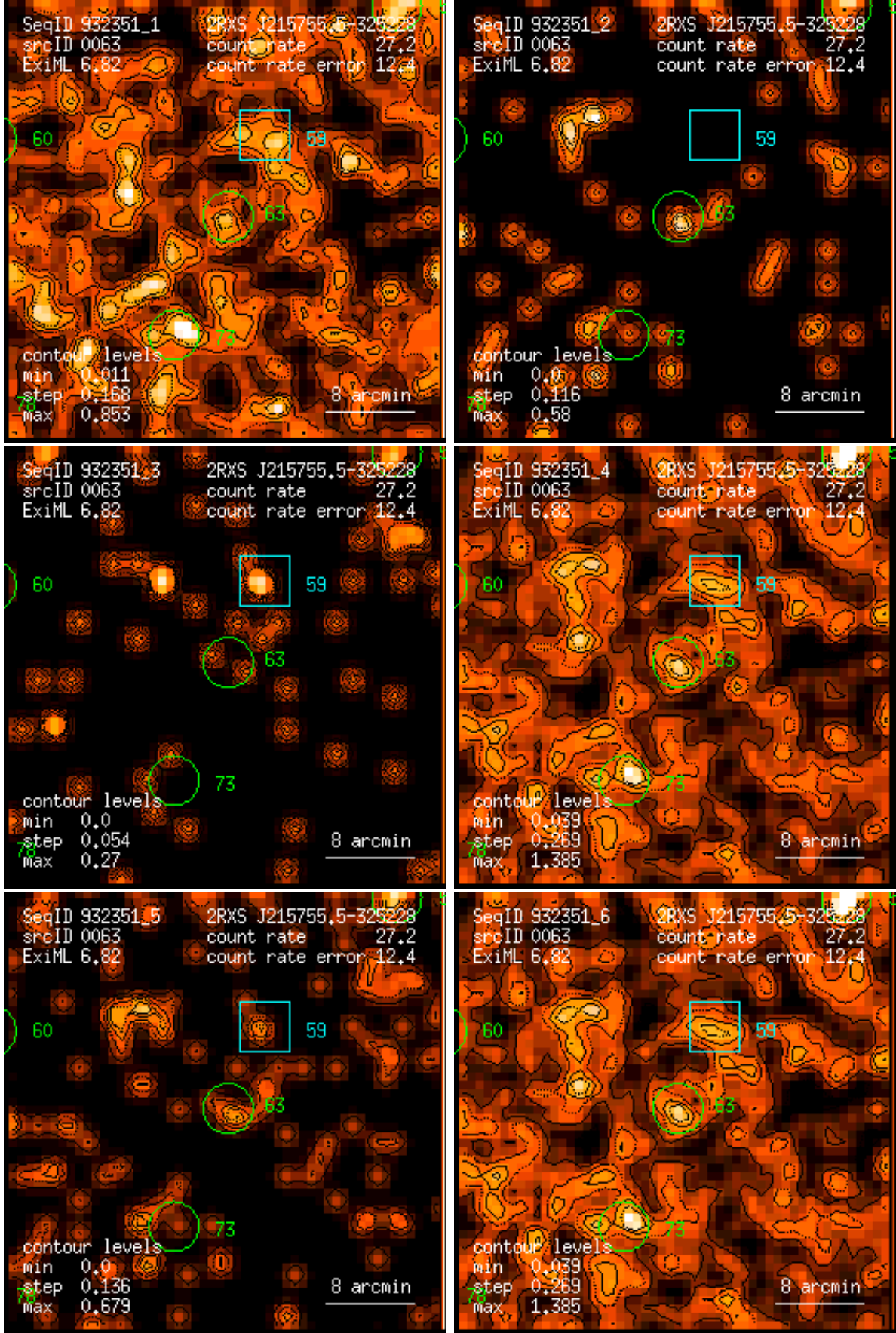
Figure 63: RASS 932351: detection 0063: band rate images, Gaussian filter: (1) PSPC channels 11 – 41, (2) 52 – 90, (3) 91 – 201, (4) 11 – 235, (5) 52 – 201, (6) 11 – 201. Broad band rates in counts/ks. Band rate contour levels in counts/ks/arcmin 2 .
