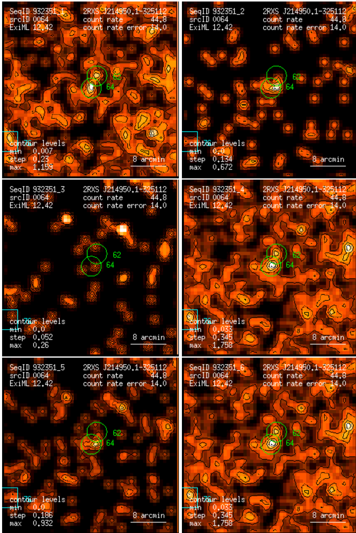
Figure 64: RASS 932351: detection 0064: band rate images, Gaussian filter: (1) PSPC channels 11 – 41, (2) 52 – 90, (3) 91 – 201, (4) 11 – 235, (5) 52 – 201, (6) 11 – 201. Broad band rates in counts/ks. Band rate contour levels in counts/ks/arcmin 2 .
