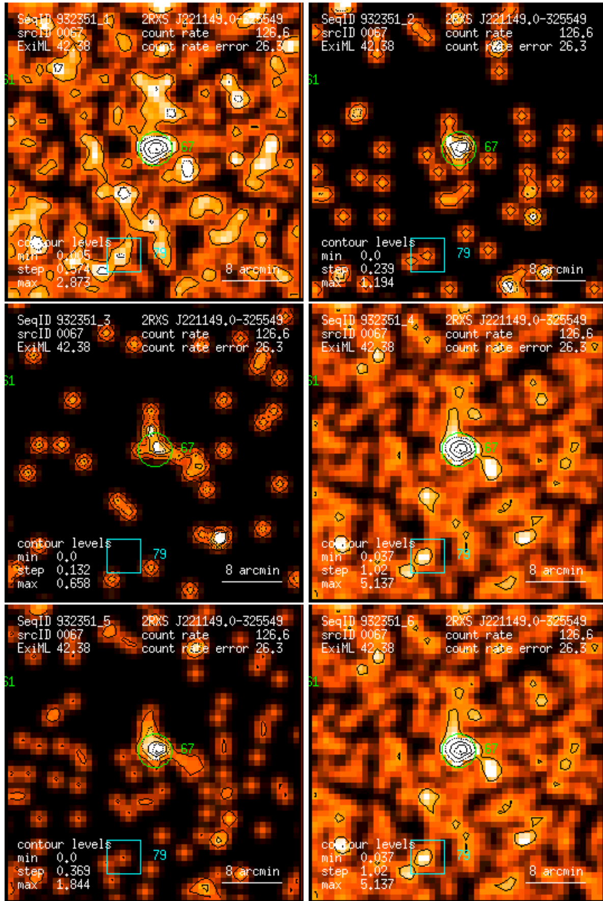
Figure 67: RASS 932351: detection 0067: band rate images, Gaussian filter: (1) PSPC channels 11 – 41, (2) 52 – 90, (3) 91 – 201, (4) 11 – 235, (5) 52 – 201, (6) 11 – 201. Broad band rates in counts/ks. Band rate contour levels in counts/ks/arcmin 2 .
