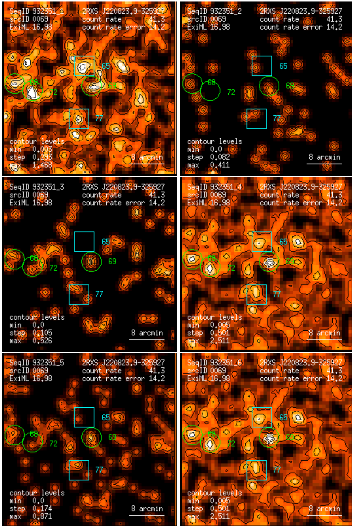
Figure 69: RASS 932351: detection 0069: band rate images, Gaussian filter: (1) PSPC channels 11 – 41, (2) 52 – 90, (3) 91 – 201, (4) 11 – 235, (5) 52 – 201, (6) 11 – 201. Broad band rates in counts/ks. Band rate contour levels in counts/ks/arcmin 2 .
