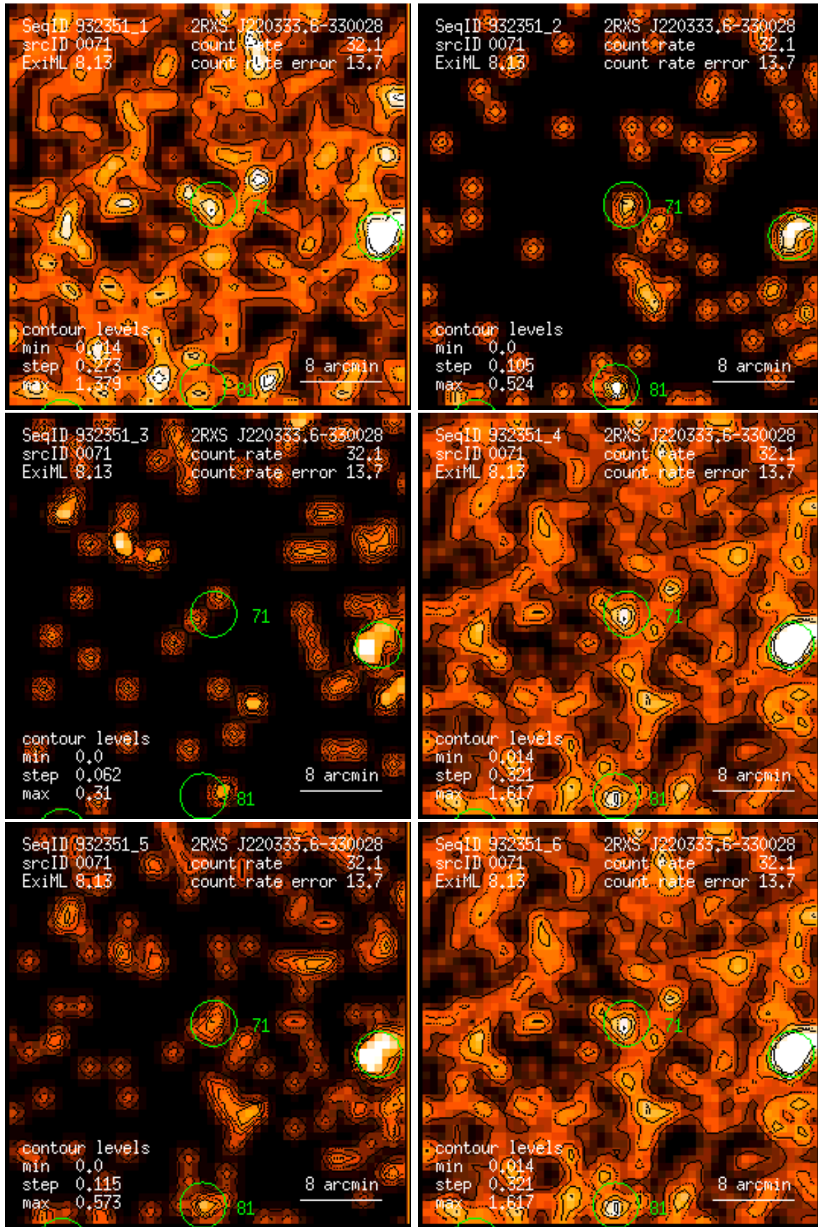
Figure 71: RASS 932351: detection 0071: band rate images, Gaussian filter: (1) PSPC channels 11 – 41, (2) 52 – 90, (3) 91 – 201, (4) 11 – 235, (5) 52 – 201, (6) 11 – 201. Broad band rates in counts/ks. Band rate contour levels in counts/ks/arcmin 2 .
