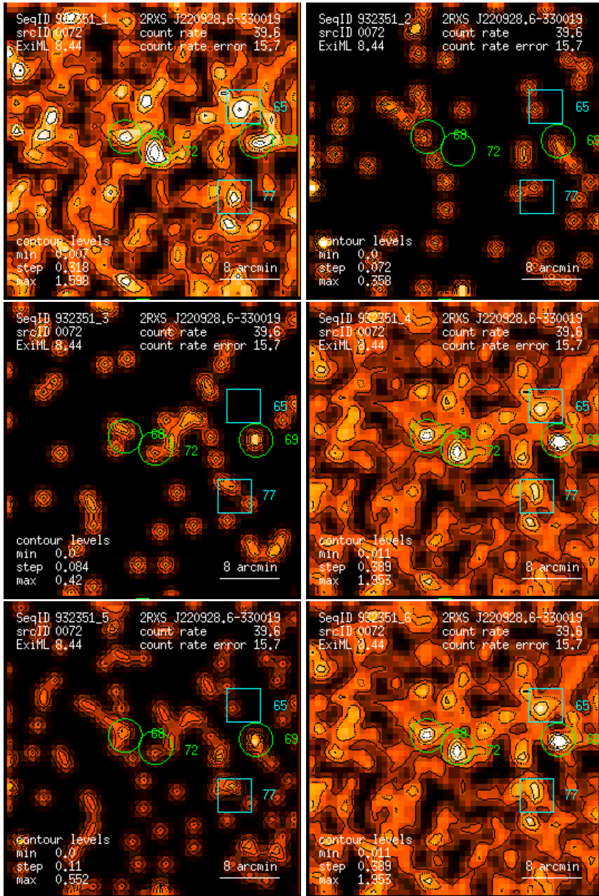
Figure 72: RASS 932351: detection 0072: band rate images, Gaussian filter: (1) PSPC channels 11 – 41, (2) 52 – 90, (3) 91 – 201, (4) 11 – 235, (5) 52 – 201, (6) 11 – 201. Broad band rates in counts/ks. Band rate contour levels in counts/ks/arcmin 2 .
