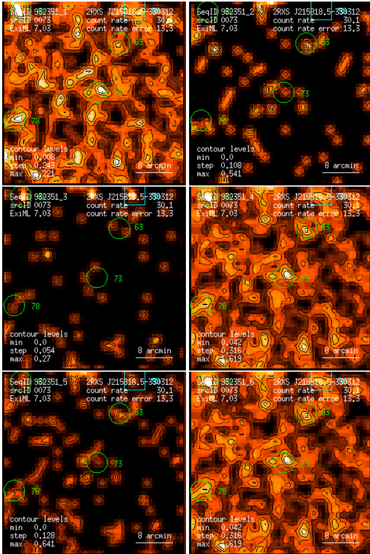
Figure 73: RASS 932351: detection 0073: band rate images, Gaussian filter: (1) PSPC channels 11 – 41, (2) 52 – 90, (3) 91 – 201, (4) 11 – 235, (5) 52 – 201, (6) 11 – 201. Broad band rates in counts/ks. Band rate contour levels in counts/ks/arcmin 2 .
