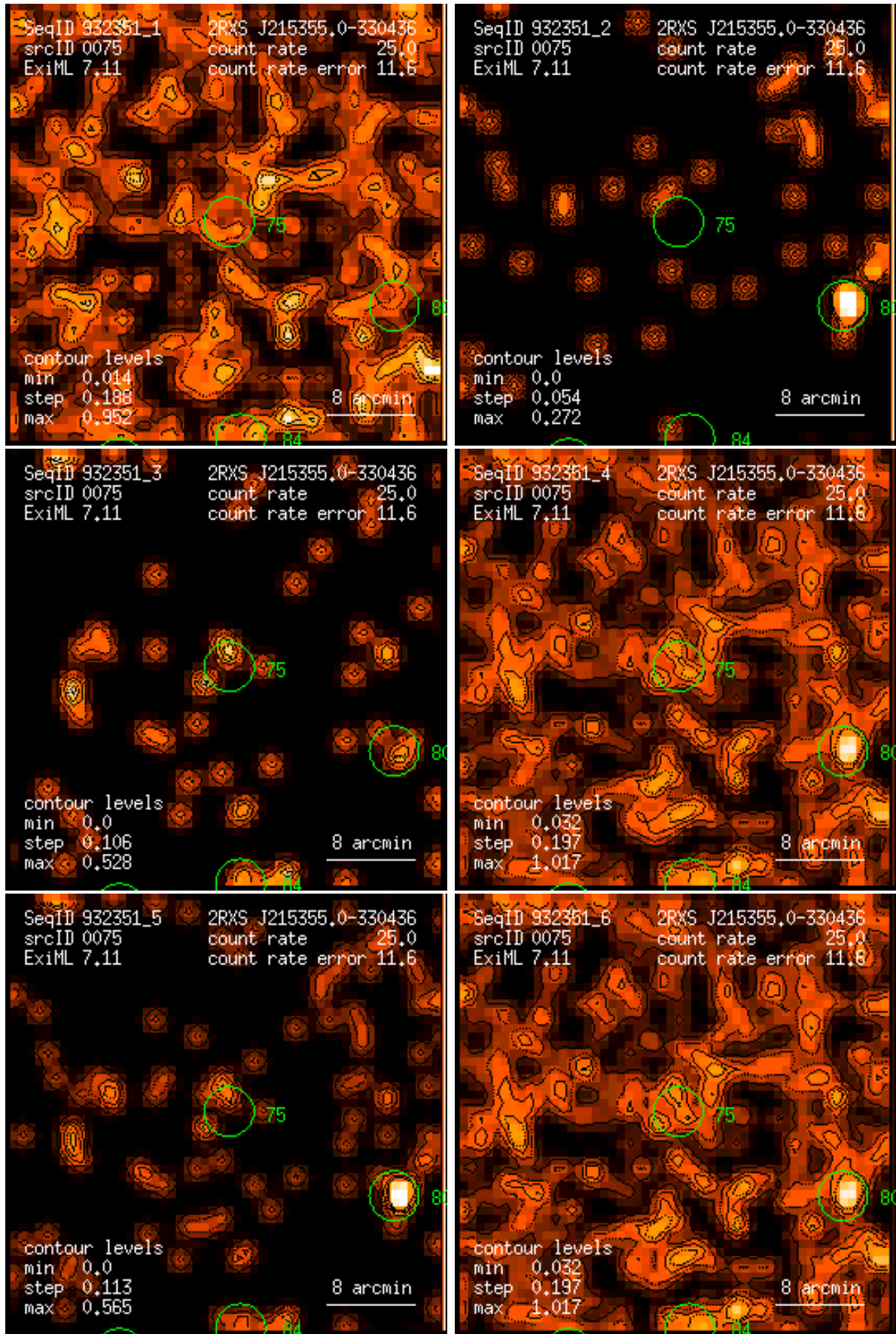
Figure 75: RASS 932351: detection 0075: band rate images, Gaussian filter: (1) PSPC channels 11 – 41, (2) 52 – 90, (3) 91 – 201, (4) 11 – 235, (5) 52 – 201, (6) 11 – 201. Broad band rates in counts/ks. Band rate contour levels in counts/ks/arcmin 2 .
