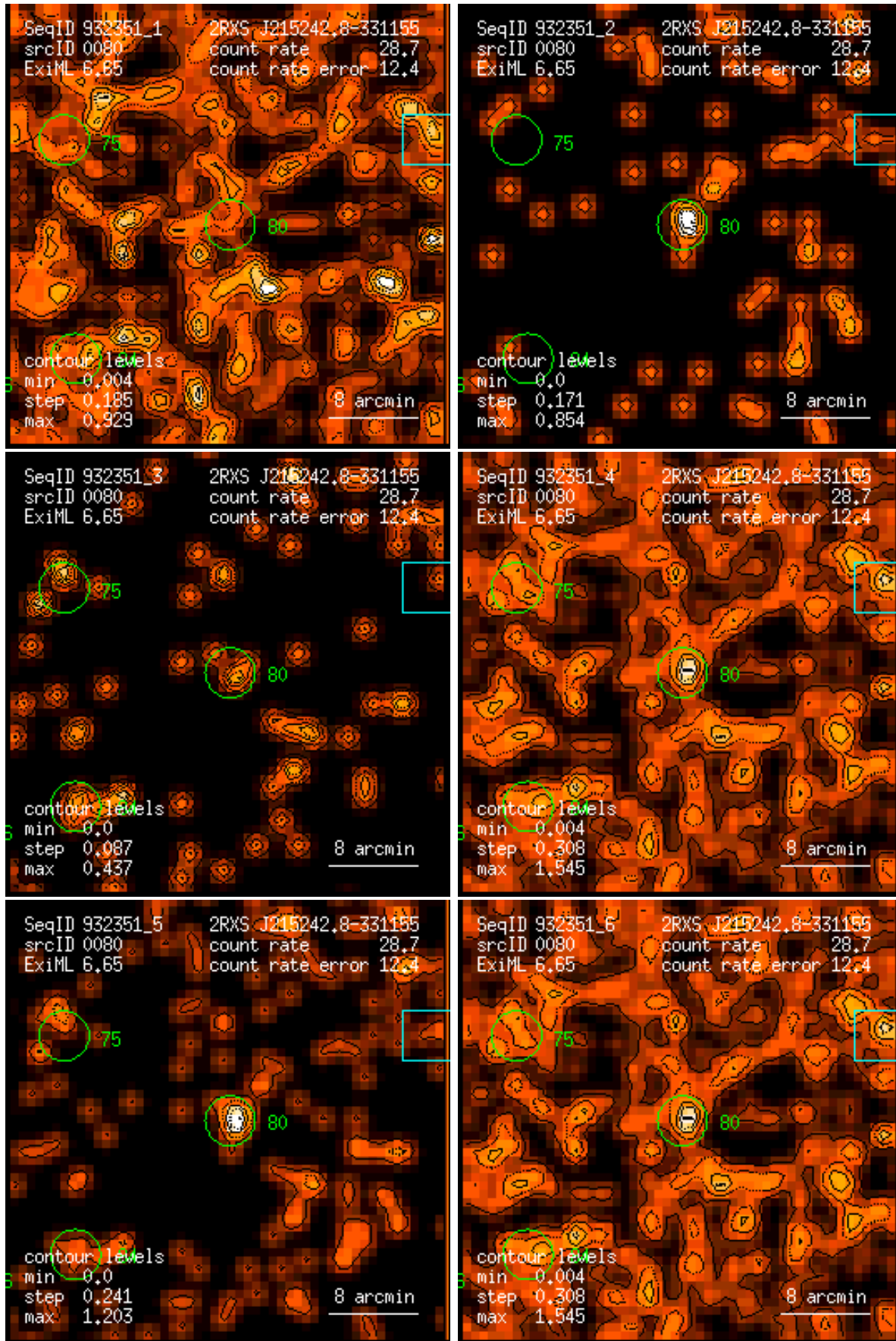
Figure 80: RASS 932351: detection 0080: band rate images, Gaussian filter: (1) PSPC channels 11 – 41, (2) 52 – 90, (3) 91 – 201, (4) 11 – 235, (5) 52 – 201, (6) 11 – 201. Broad band rates in counts/ks. Band rate contour levels in counts/ks/arcmin 2 .
