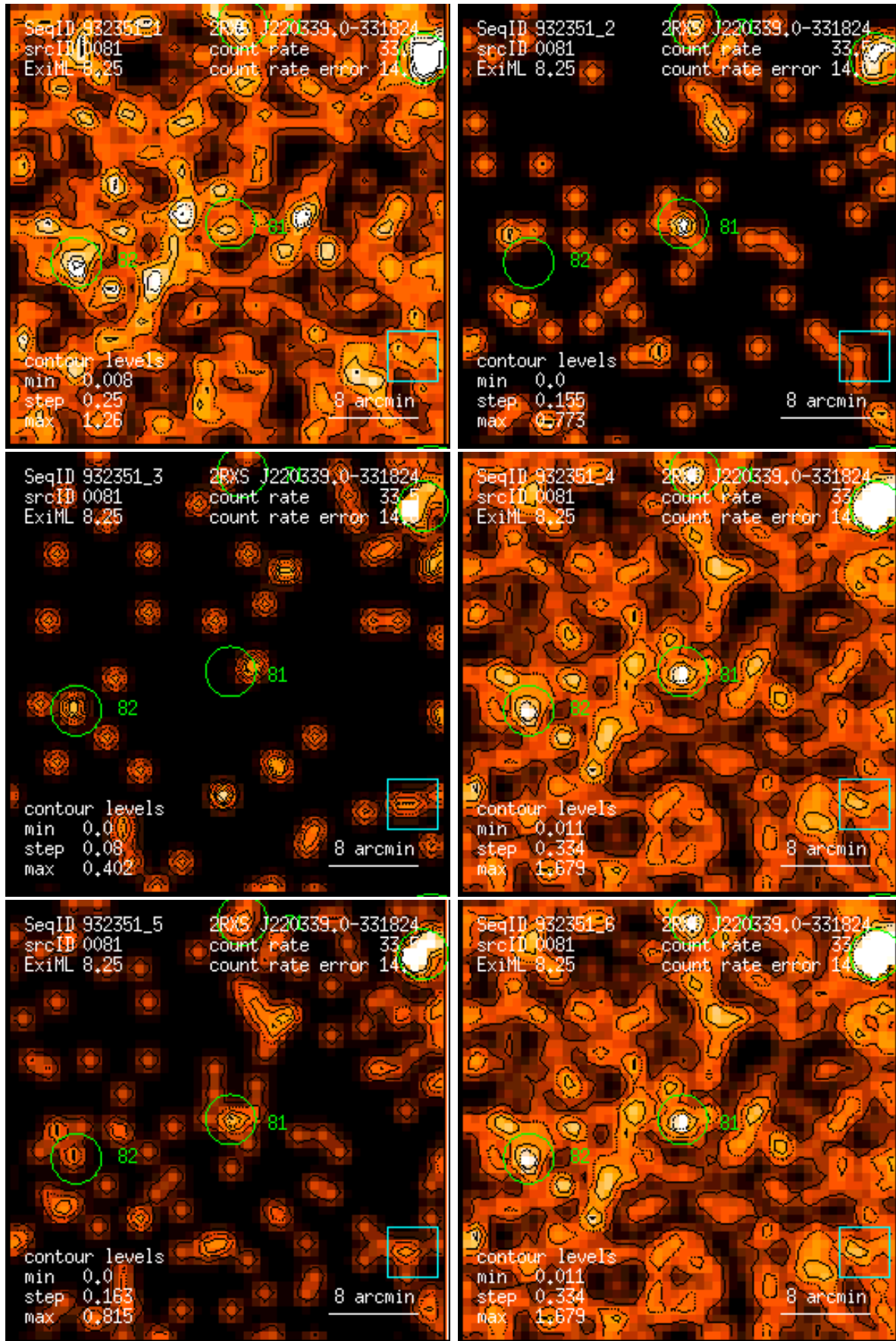
Figure 81: RASS 932351: detection 0081: band rate images, Gaussian filter: (1) PSPC channels 11 – 41, (2) 52 – 90, (3) 91 – 201, (4) 11 – 235, (5) 52 – 201, (6) 11 – 201. Broad band rates in counts/ks. Band rate contour levels in counts/ks/arcmin 2 .
