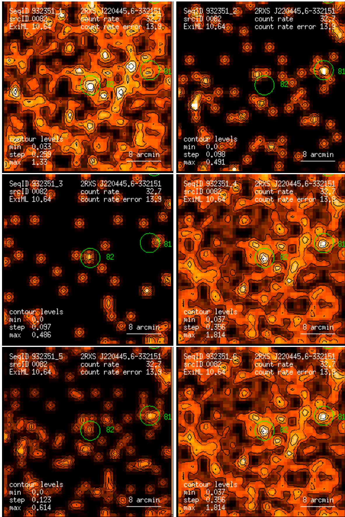
Figure 82: RASS 932351: detection 0082: band rate images, Gaussian filter: (1) PSPC channels 11 – 41, (2) 52 – 90, (3) 91 – 201, (4) 11 – 235, (5) 52 – 201, (6) 11 – 201. Broad band rates in counts/ks. Band rate contour levels in counts/ks/arcmin 2 .
