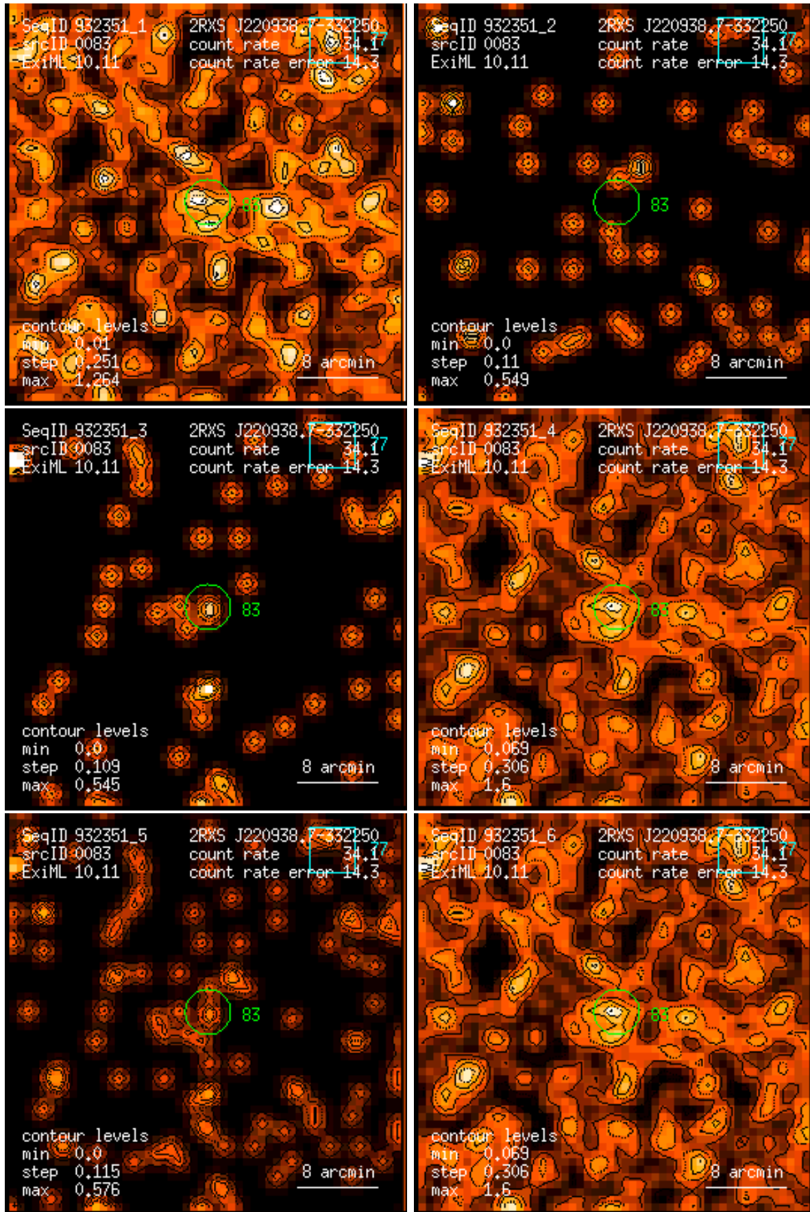
Figure 83: RASS 932351: detection 0083: band rate images, Gaussian filter: (1) PSPC channels 11 – 41, (2) 52 – 90, (3) 91 – 201, (4) 11 – 235, (5) 52 – 201, (6) 11 – 201. Broad band rates in counts/ks. Band rate contour levels in counts/ks/arcmin 2 .
