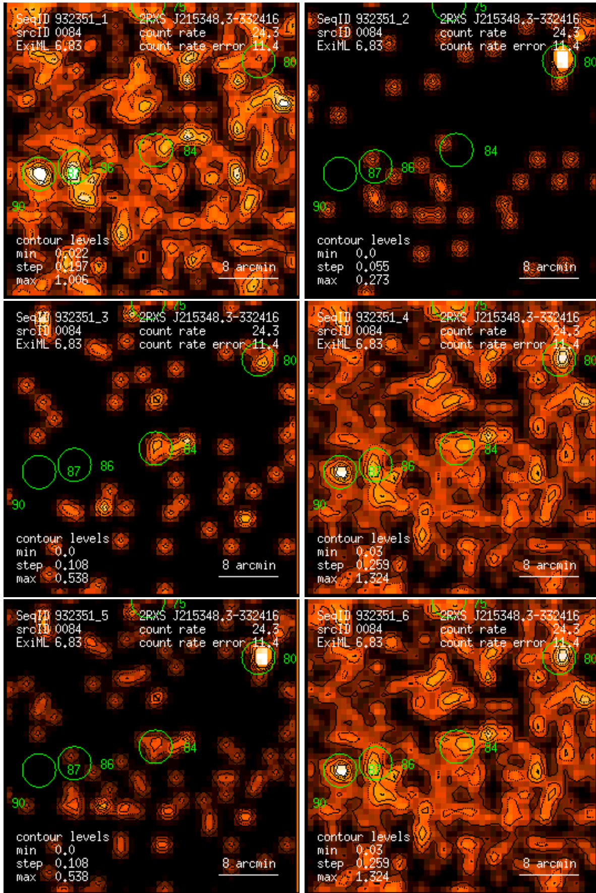
Figure 84: RASS 932351: detection 0084: band rate images, Gaussian filter: (1) PSPC channels 11 – 41, (2) 52 – 90, (3) 91 – 201, (4) 11 – 235, (5) 52 – 201, (6) 11 – 201. Broad band rates in counts/ks. Band rate contour levels in counts/ks/arcmin 2 .
