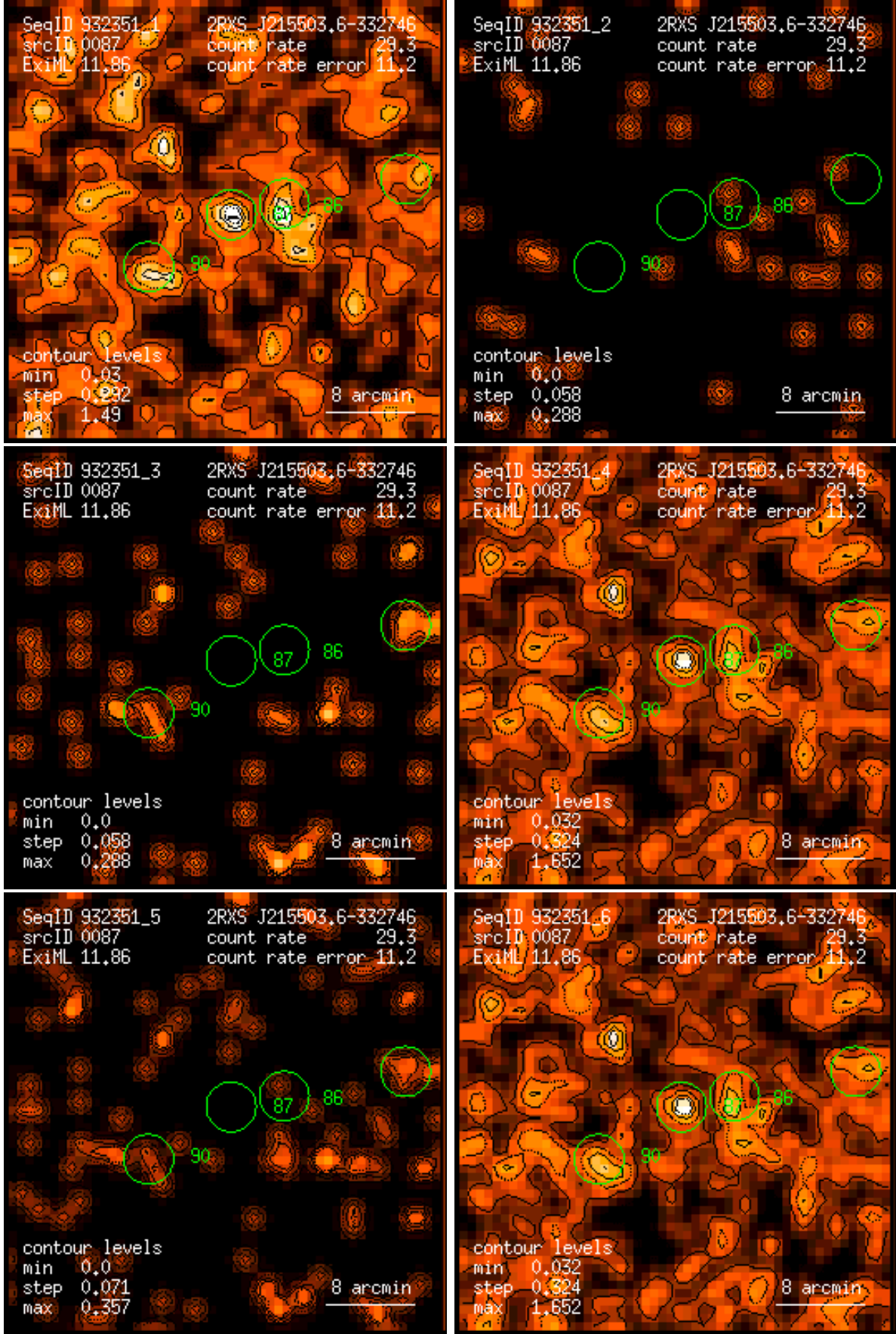
Figure 87: RASS 932351: detection 0087: band rate images, Gaussian filter: (1) PSPC channels 11 – 41, (2) 52 – 90, (3) 91 – 201, (4) 11 – 235, (5) 52 – 201, (6) 11 – 201. Broad band rates in counts/ks. Band rate contour levels in counts/ks/arcmin 2 .
