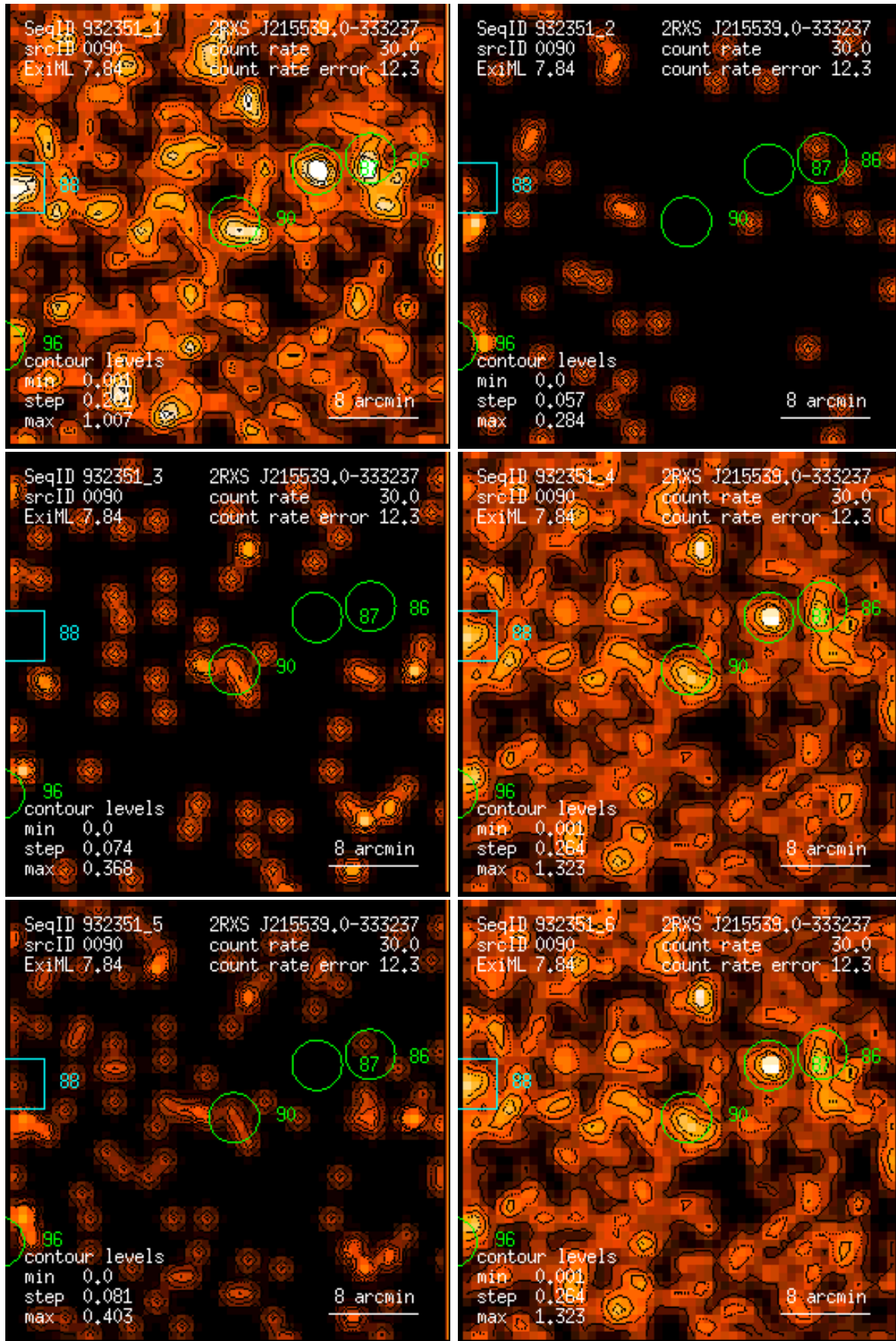
Figure 90: RASS 932351: detection 0090: band rate images, Gaussian filter: (1) PSPC channels 11 – 41, (2) 52 – 90, (3) 91 – 201, (4) 11 – 235, (5) 52 – 201, (6) 11 – 201. Broad band rates in counts/ks. Band rate contour levels in counts/ks/arcmin 2 .
