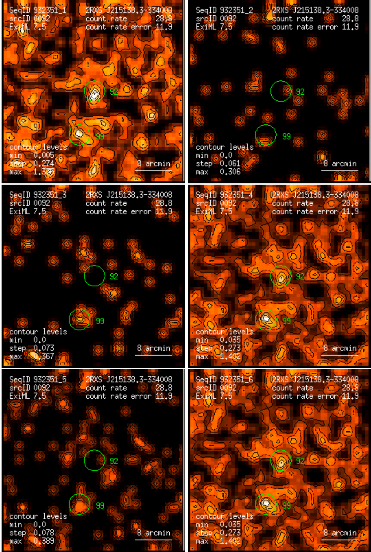
Figure 92: RASS 932351: detection 0092: band rate images, Gaussian filter: (1) PSPC channels 11 – 41, (2) 52 – 90, (3) 91 – 201, (4) 11 – 235, (5) 52 – 201, (6) 11 – 201. Broad band rates in counts/ks. Band rate contour levels in counts/ks/arcmin 2 .
