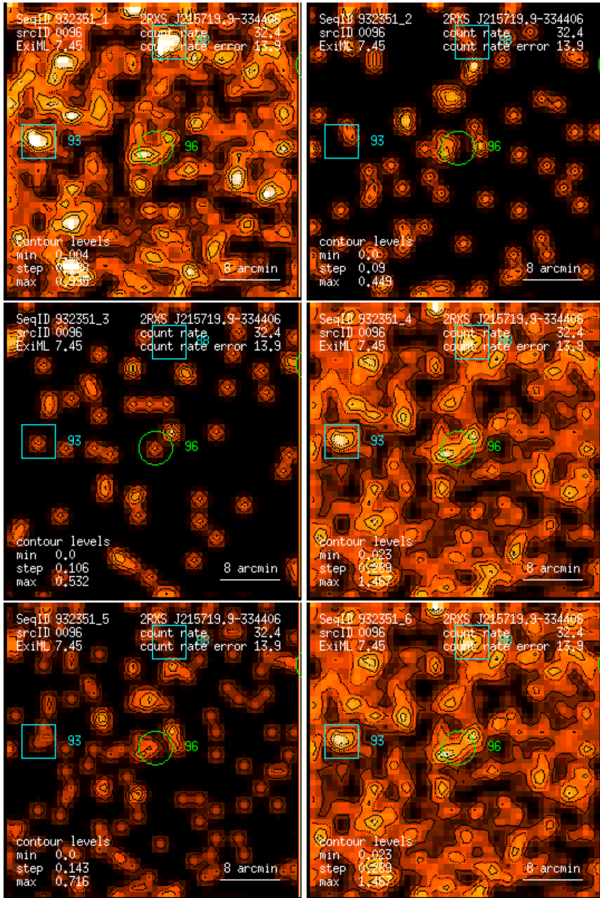
Figure 96: RASS 932351: detection 0096: band rate images, Gaussian filter: (1) PSPC channels 11 – 41, (2) 52 – 90, (3) 91 – 201, (4) 11 – 235, (5) 52 – 201, (6) 11 – 201. Broad band rates in counts/ks. Band rate contour levels in counts/ks/arcmin 2 .
