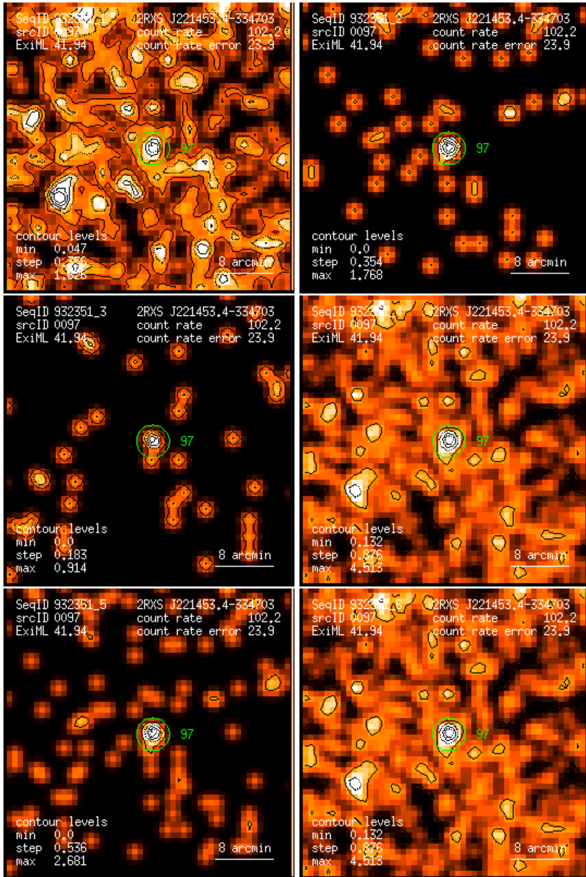
Figure 97: RASS 932351: detection 0097: band rate images, Gaussian filter: (1) PSPC channels 11 – 41, (2) 52 – 90, (3) 91 – 201, (4) 11 – 235, (5) 52 – 201, (6) 11 – 201. Broad band rates in counts/ks. Band rate contour levels in counts/ks/arcmin 2 .
