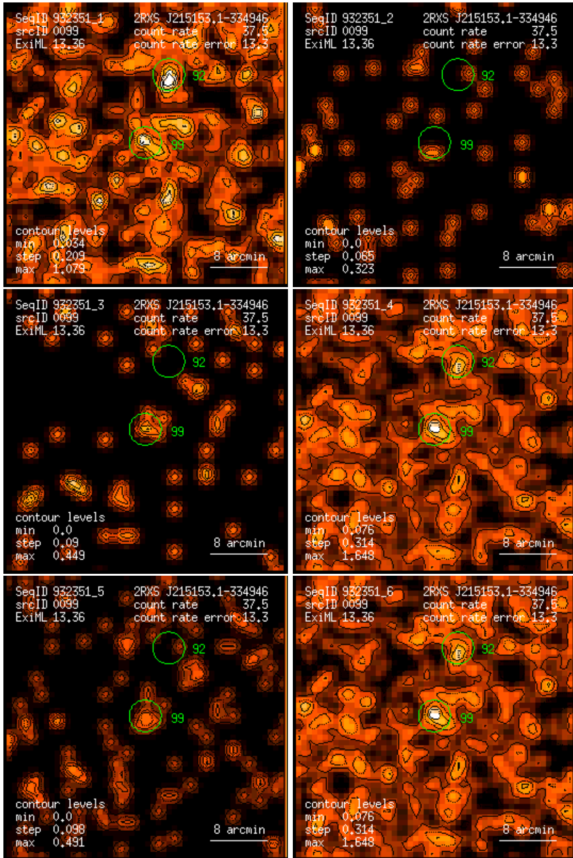
Figure 99: RASS 932351: detection 0099: band rate images, Gaussian filter: (1) PSPC channels 11 – 41, (2) 52 – 90, (3) 91 – 201, (4) 11 – 235, (5) 52 – 201, (6) 11 – 201. Broad band rates in counts/ks. Band rate contour levels in counts/ks/arcmin 2 .
