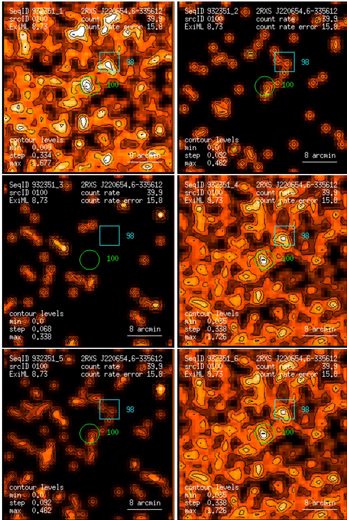
Figure 100: RASS 932351: detection 0100: band rate images, Gaussian filter: (1) PSPC channels 11 – 41, (2) 52 – 90, (3) 91 – 201, (4) 11 – 235, (5) 52 – 201, (6) 11 – 201. Broad band rates in counts/ks. Band rate contour levels in counts/ks/arcmin 2 .
