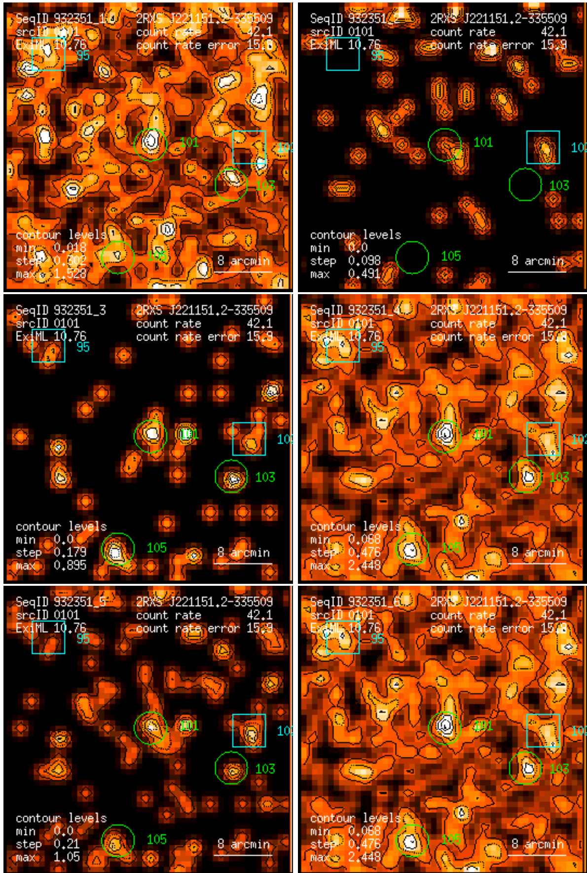
Figure 101: RASS 932351: detection 0101: band rate images, Gaussian filter: (1) PSPC channels 11 – 41, (2) 52 – 90, (3) 91 – 201, (4) 11 – 235, (5) 52 – 201, (6) 11 – 201. Broad band rates in counts/ks. Band rate contour levels in counts/ks/arcmin 2 .
