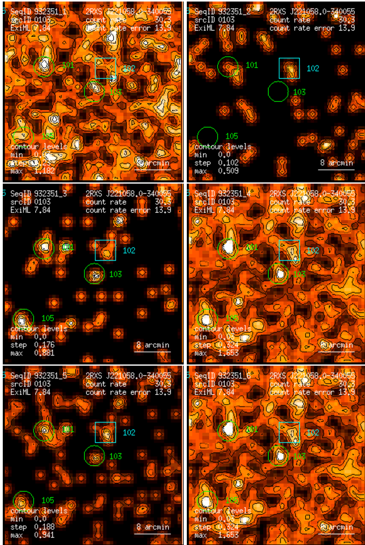
Figure 103: RASS 932351: detection 0103: band rate images, Gaussian filter: (1) PSPC channels 11 – 41, (2) 52 – 90, (3) 91 – 201, (4) 11 – 235, (5) 52 – 201, (6) 11 – 201. Broad band rates in counts/ks. Band rate contour levels in counts/ks/arcmin 2 .
