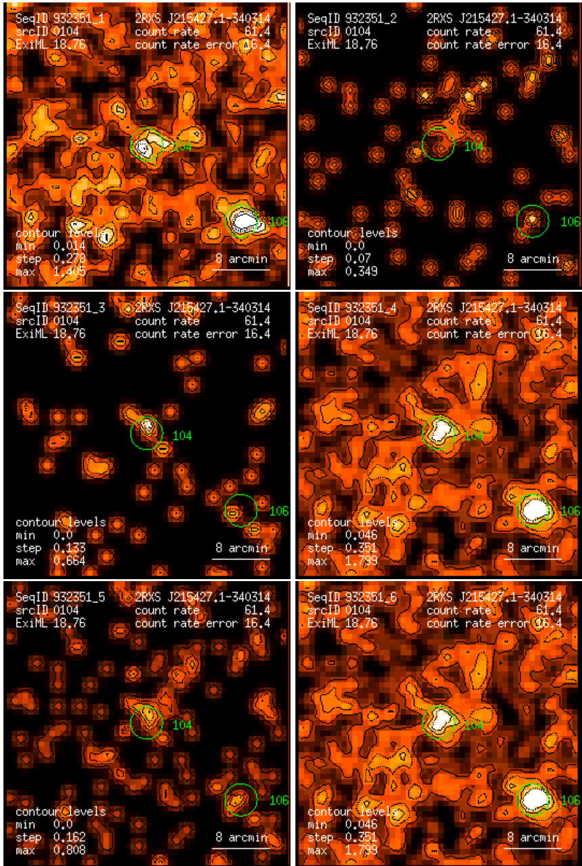
Figure 104: RASS 932351: detection 0104: band rate images, Gaussian filter: (1) PSPC channels 11 – 41, (2) 52 – 90, (3) 91 – 201, (4) 11 – 235, (5) 52 – 201, (6) 11 – 201. Broad band rates in counts/ks. Band rate contour levels in counts/ks/arcmin 2 .
