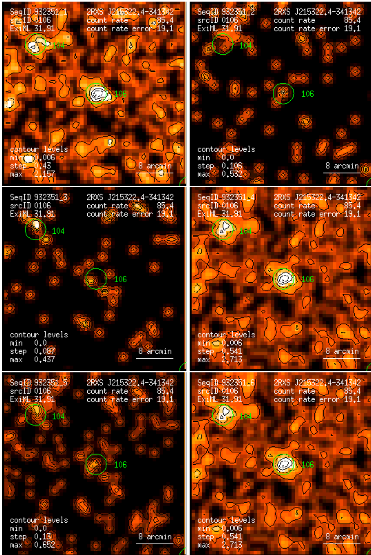
Figure 106: RASS 932351: detection 0106: band rate images, Gaussian filter: (1) PSPC channels 11 – 41, (2) 52 – 90, (3) 91 – 201, (4) 11 – 235, (5) 52 – 201, (6) 11 – 201. Broad band rates in counts/ks. Band rate contour levels in counts/ks/arcmin 2 .
