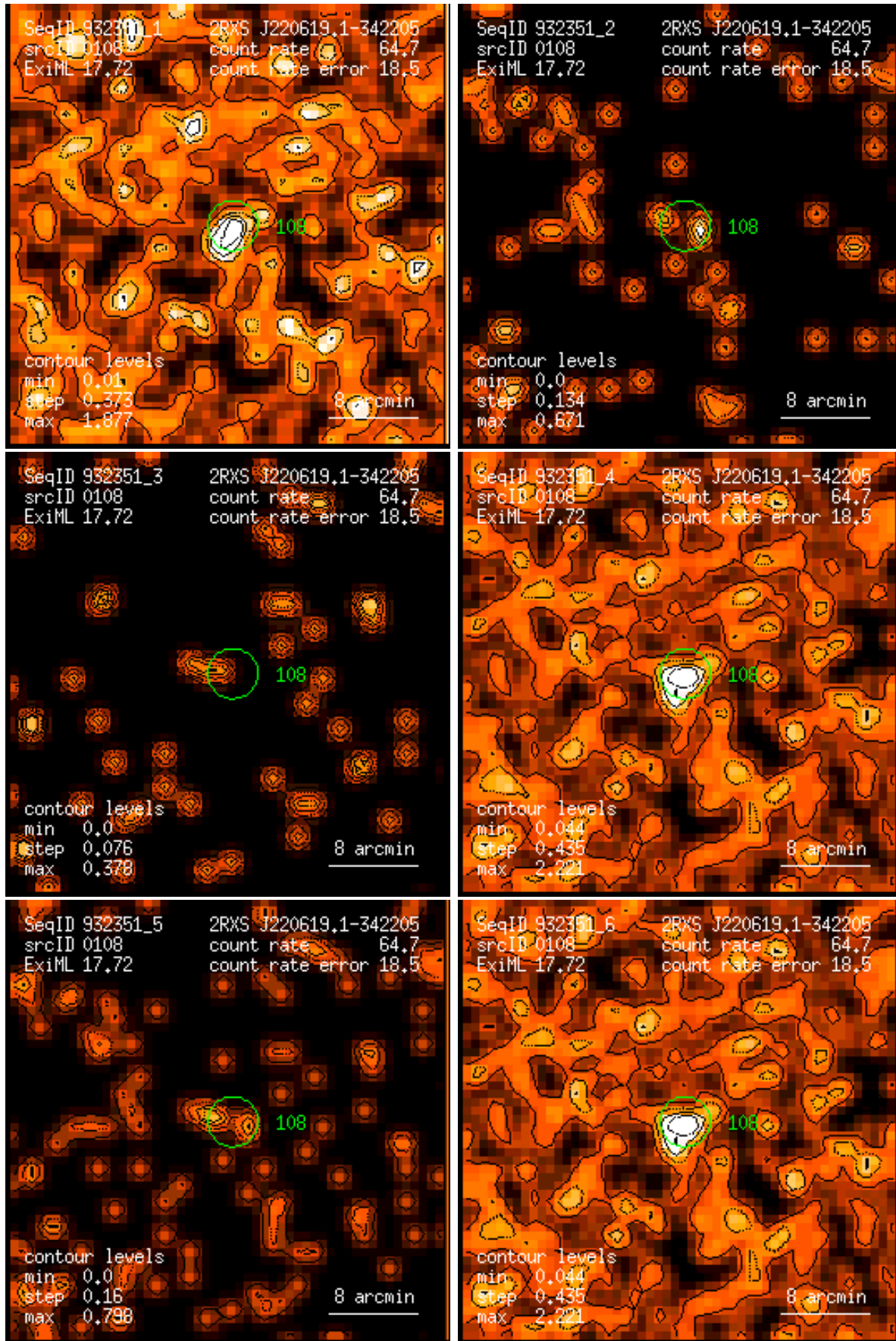
Figure 108: RASS 932351: detection 0108: band rate images, Gaussian filter: (1) PSPC channels 11 – 41, (2) 52 – 90, (3) 91 – 201, (4) 11 – 235, (5) 52 – 201, (6) 11 – 201. Broad band rates in counts/ks. Band rate contour levels in counts/ks/arcmin 2 .
