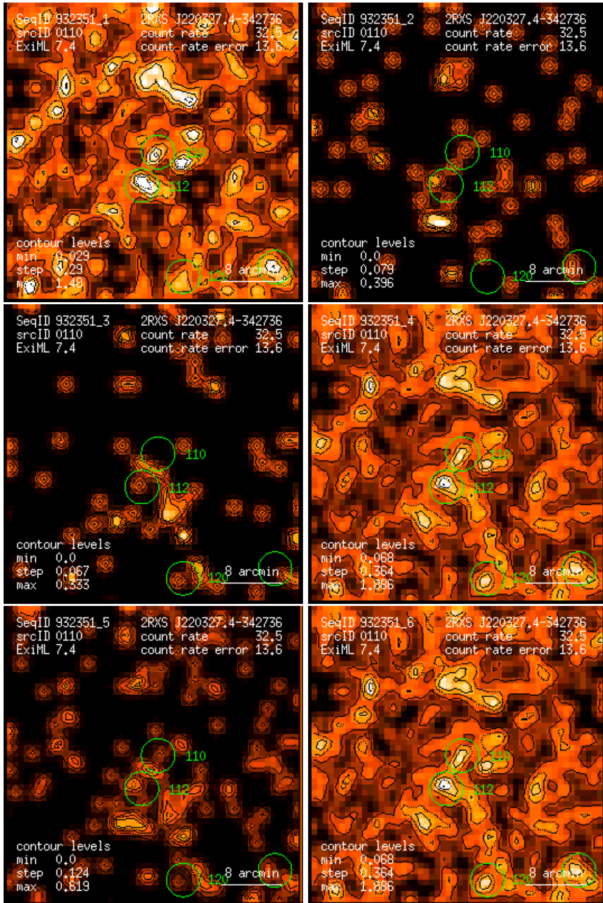
Figure 110: RASS 932351: detection 0110: band rate images, Gaussian filter: (1) PSPC channels 11 – 41, (2) 52 – 90, (3) 91 – 201, (4) 11 – 235, (5) 52 – 201, (6) 11 – 201. Broad band rates in counts/ks. Band rate contour levels in counts/ks/arcmin 2 .
