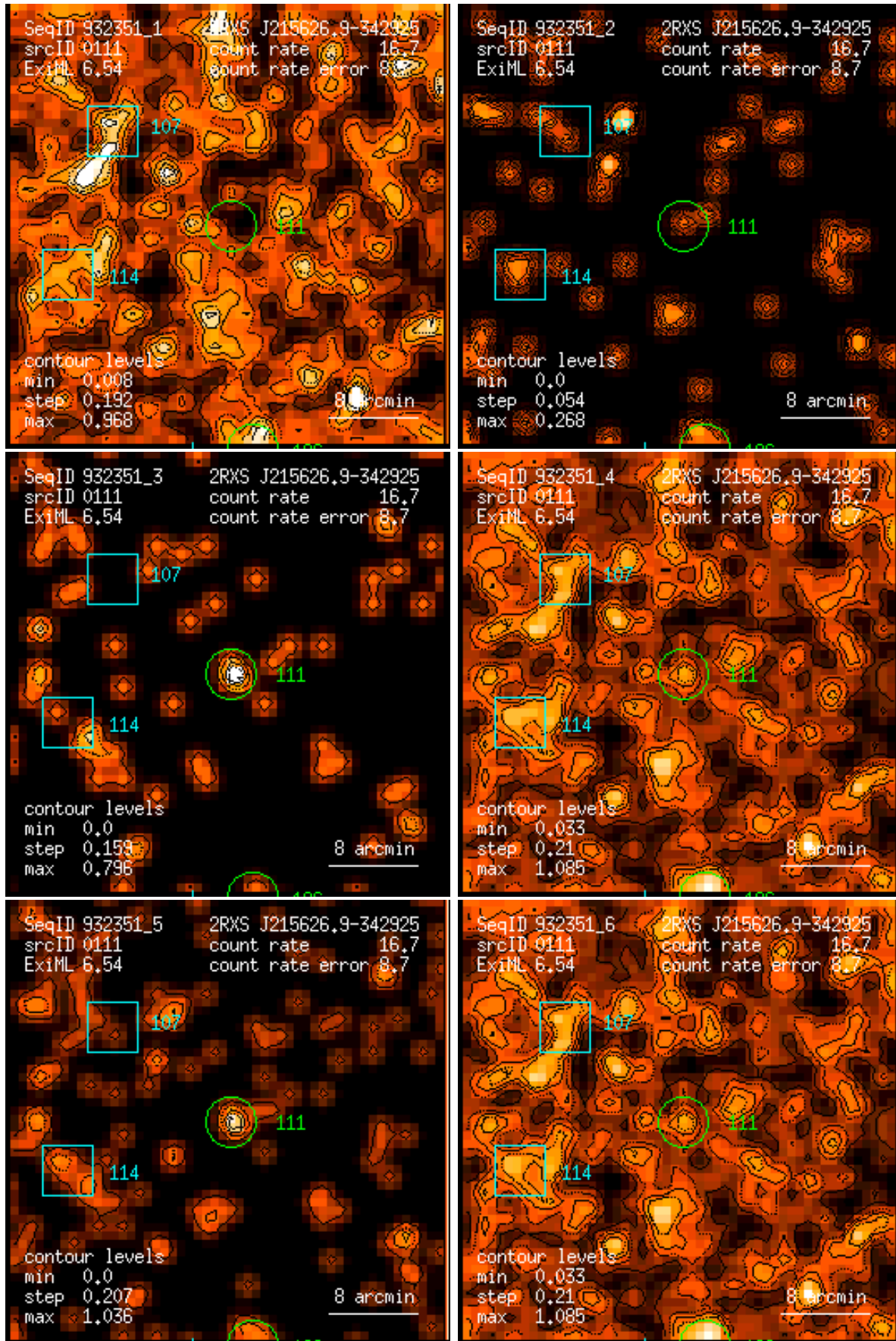
Figure 111: RASS 932351: detection 0111: band rate images, Gaussian filter: (1) PSPC channels 11 – 41, (2) 52 – 90, (3) 91 – 201, (4) 11 – 235, (5) 52 – 201, (6) 11 – 201. Broad band rates in counts/ks. Band rate contour levels in counts/ks/arcmin 2 .
